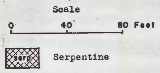
Plate 5, Figure 1 OUTCROP GEOLOGIC MAP OF THE NORTH TALC PROSPECT, BETWEEN HOOSAC TUNNEL AND DRURY, MASSACHUSETTS
