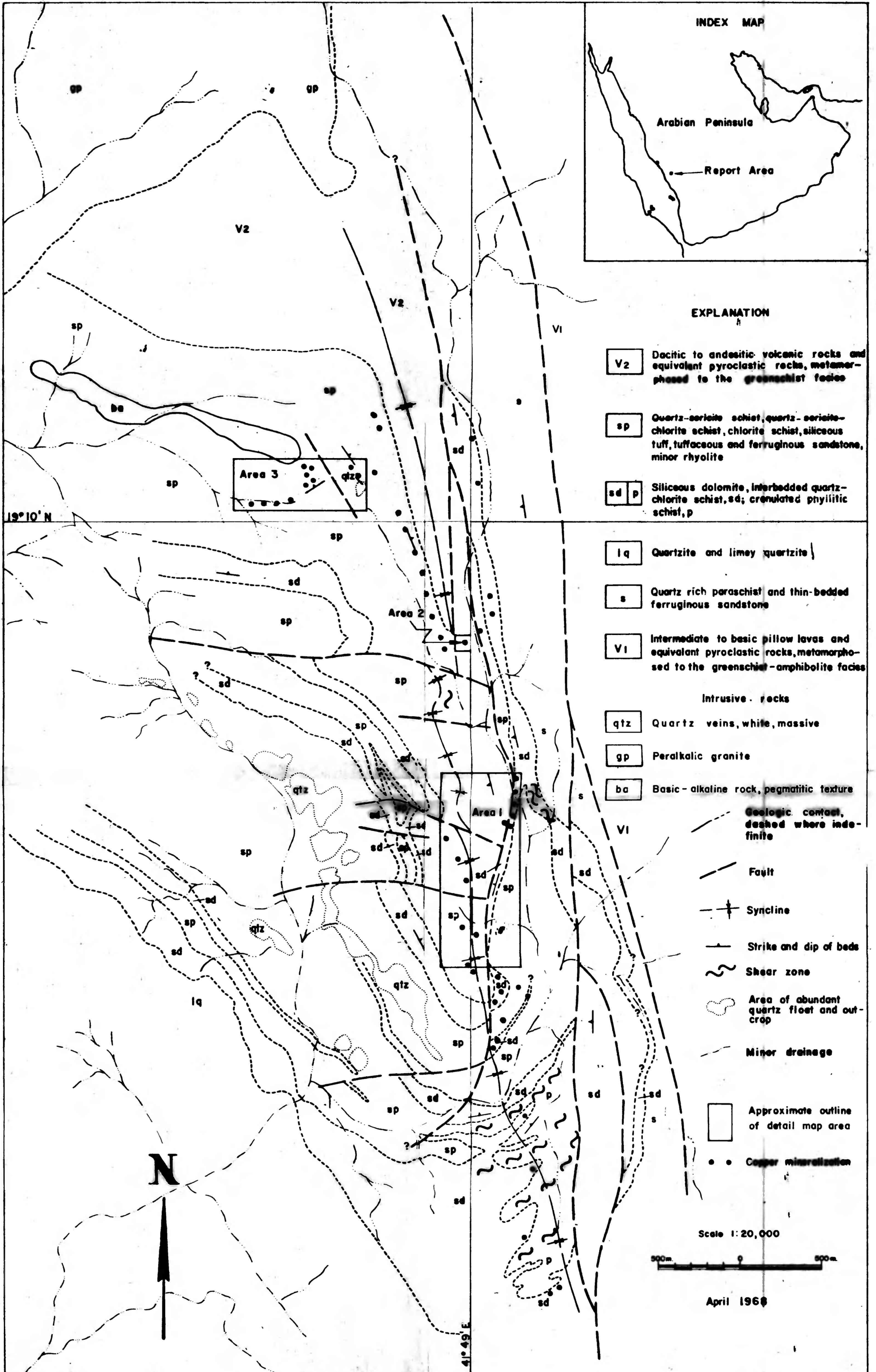
FIGURE 1.- Geologic map of the Wadi Yiba copper prospect
