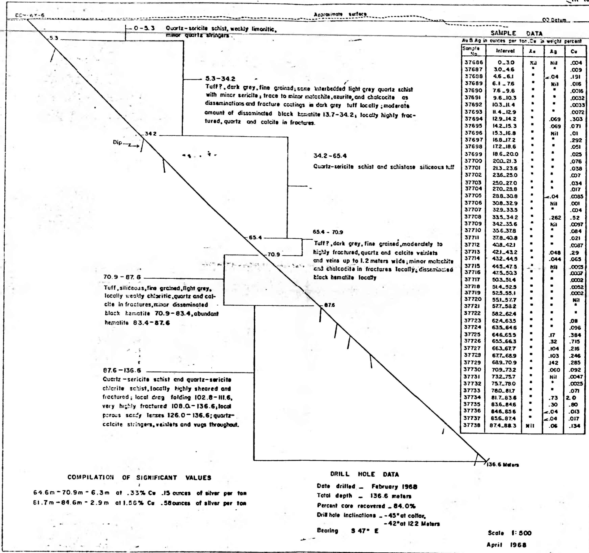
FIGURE 9.- Section, diamond drill hole WY-6, looking Northeast
