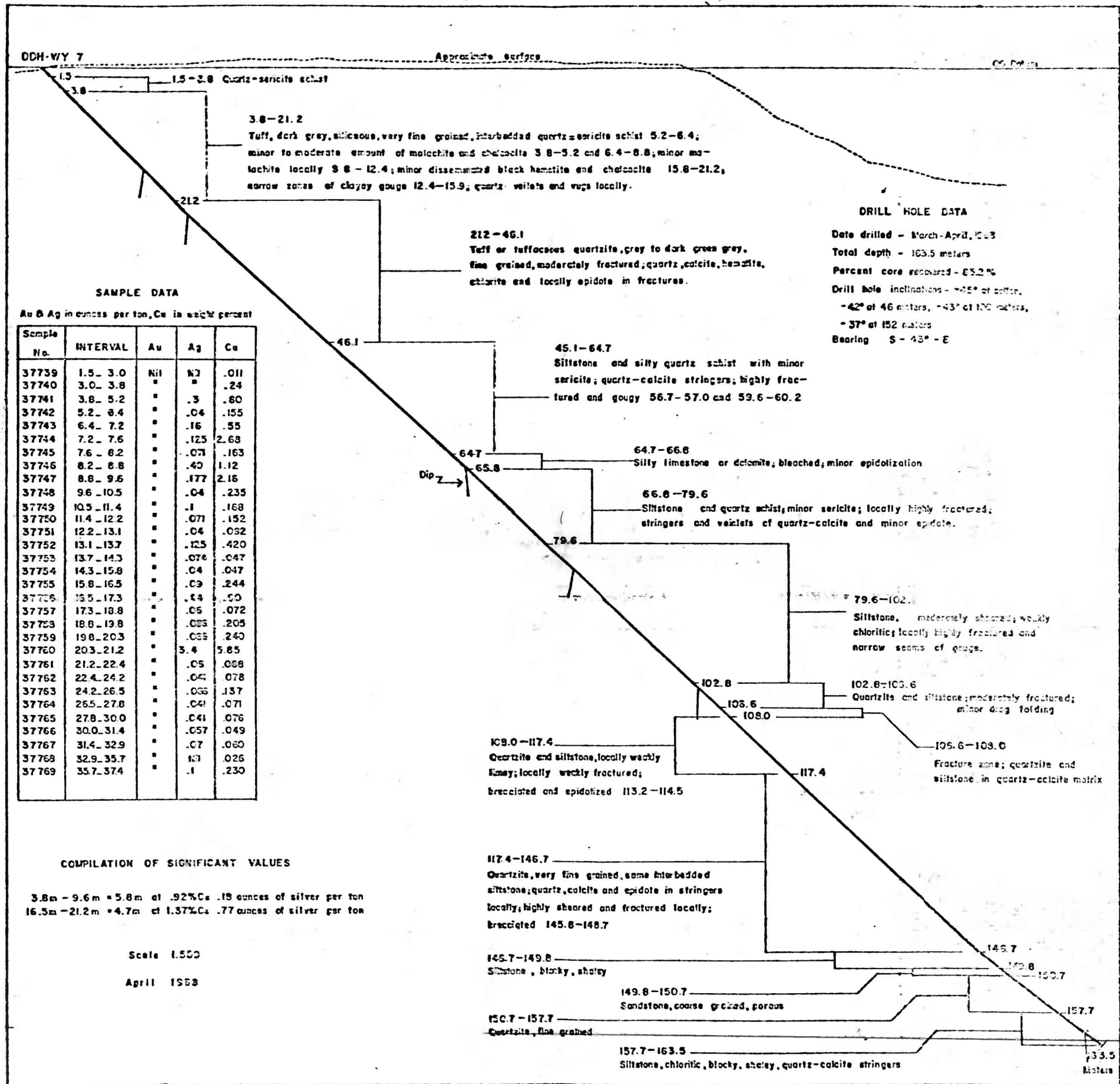
FIGURE 10 - Section, diamond drill hole WY-7, looking Northeast
