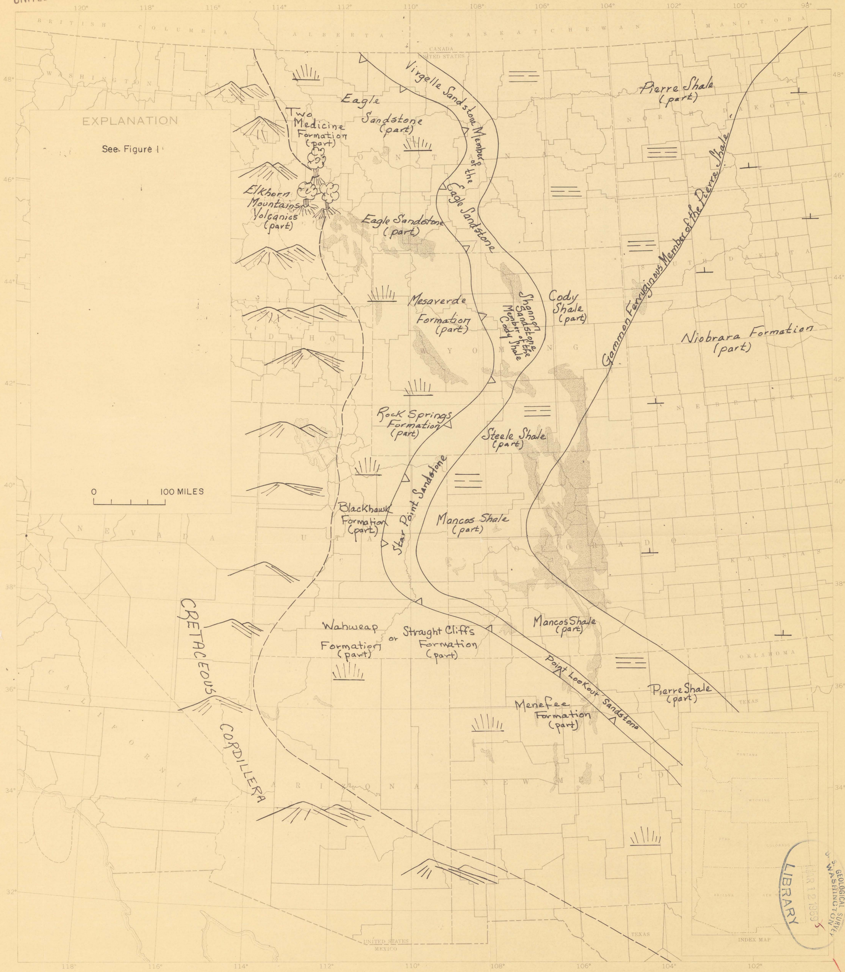
FIGURE 2.-- PALEOGEOGRAPHIC MAP FOR LATEST EAGLE TIME SHOWING POSITION OF STRANDLINE DURING RANGE ZONE OF BACULITES SP (SMOOTH FORM) BY
