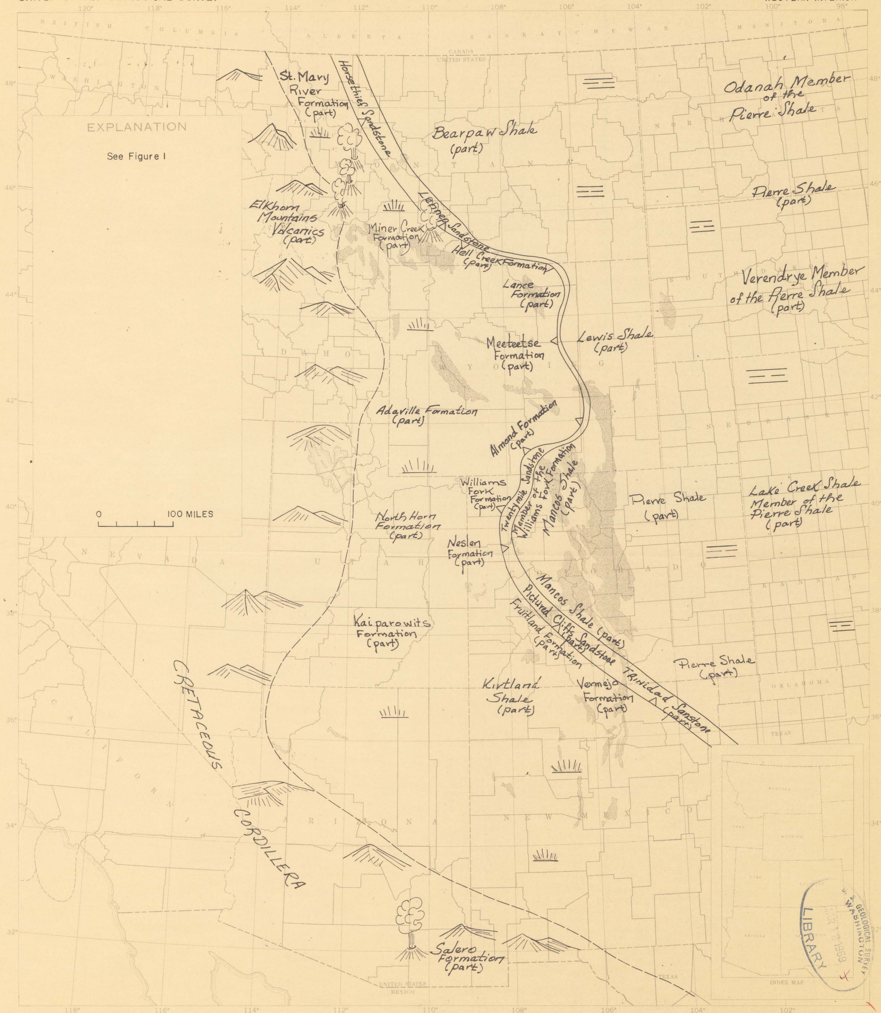
FIGURE 5.-- PALEOGEOGRAPHIC MAP FOR MIDDLE BEARPAW TIME SHOWING POSITION OF STRANDLINE DURING RANGE ZONE OF BACULITES REESIDE
