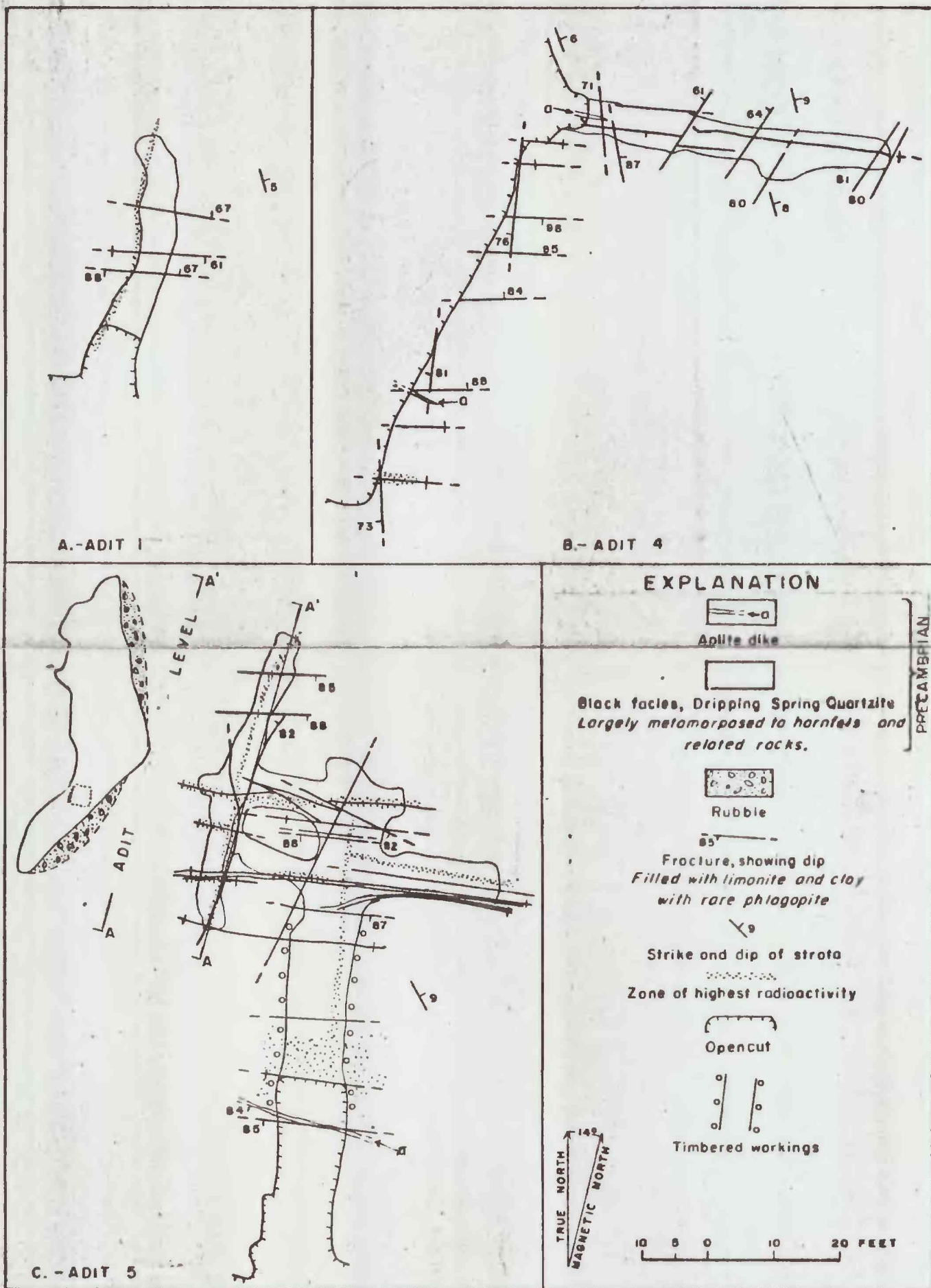
FIGURE 4.--GEOLOGIC MAPS OF ADITS 1, 4, AND 5, LITTLE JOE DEPOSITS
