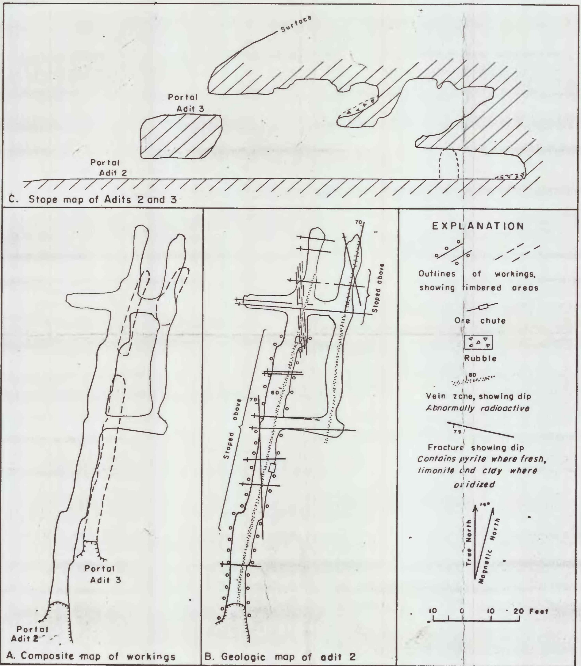
FIGURE 5.--GEOLOGIC MAPS AND SECTION OF ADITS 2 AND 3, LITTLE JOE DEPOSITS
