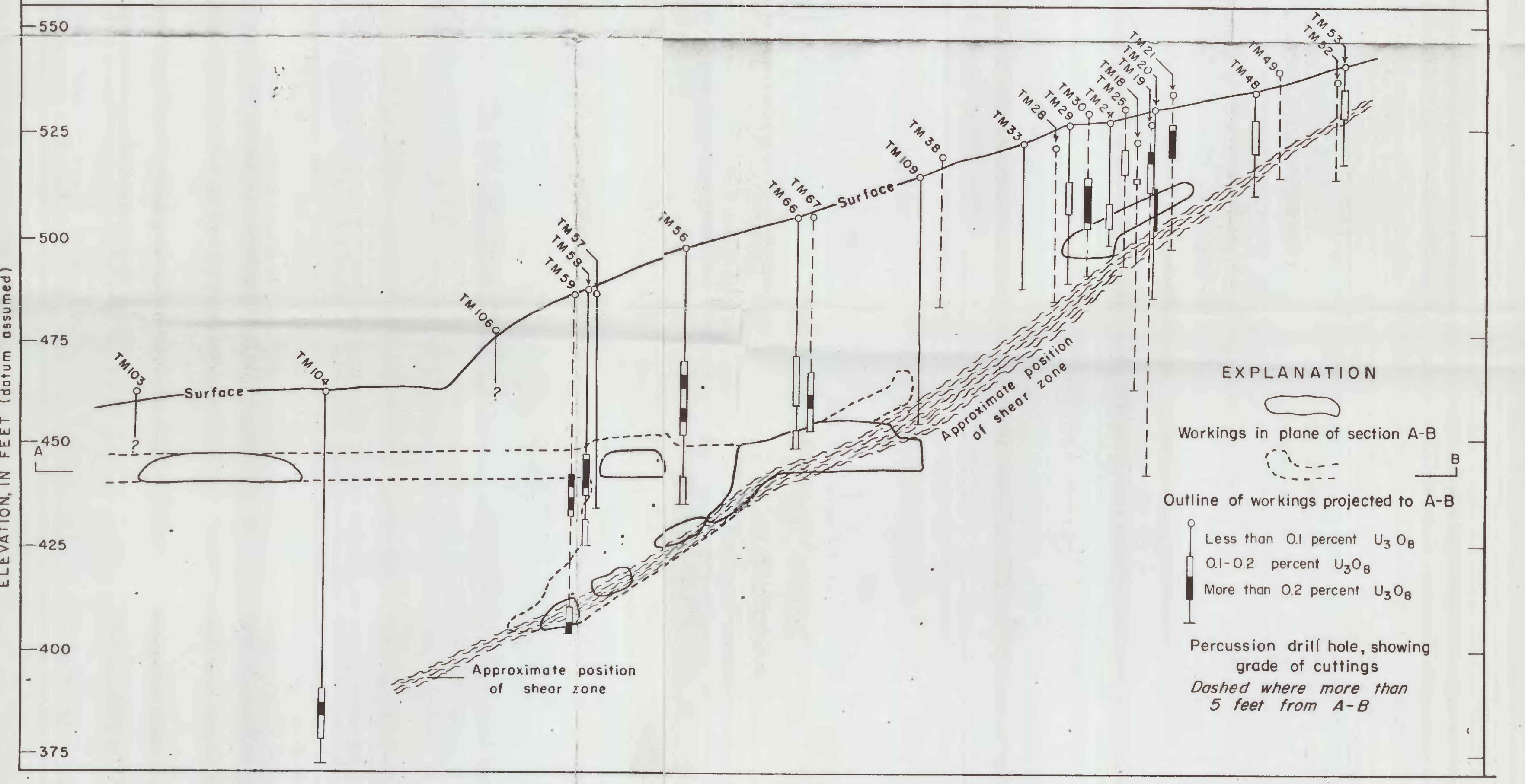
FIGURE 6.-- MAP AND SECTION OF WORKINGS AND DRILL HOLES, LUCKY BOY MINE, GILA COUNTY, ARIZONA
