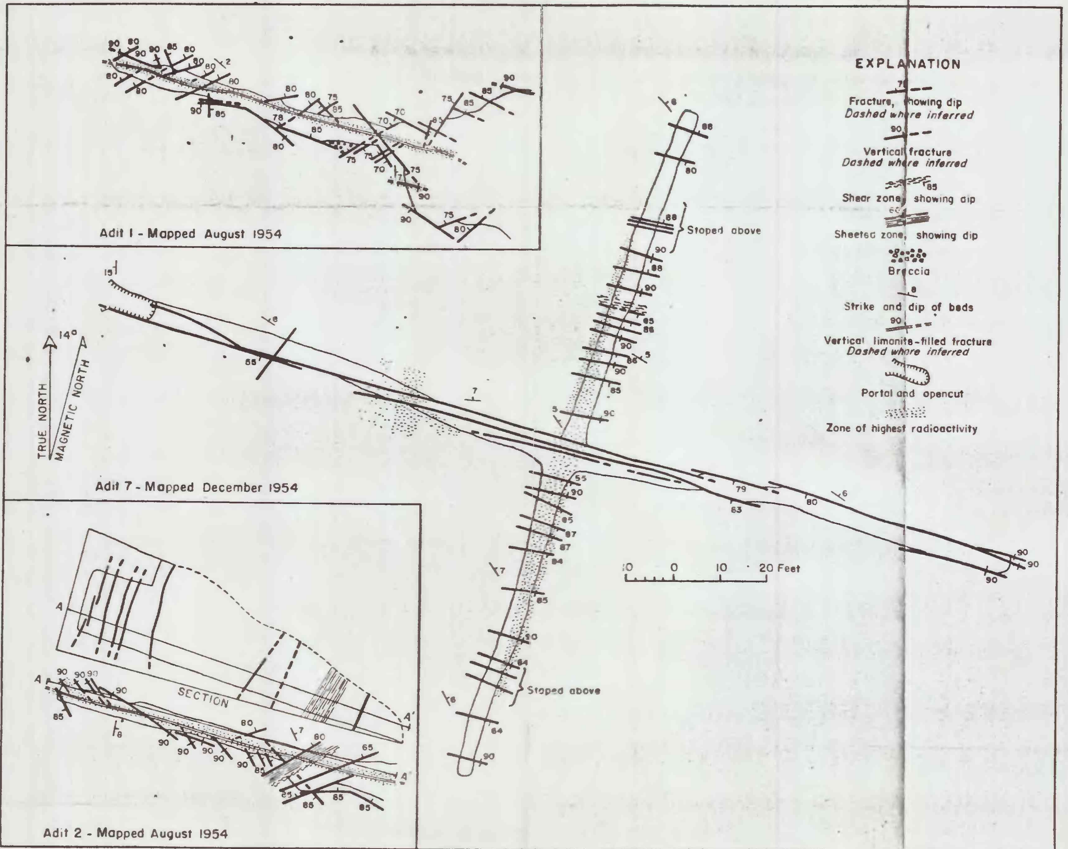
FIGURE 7.--GEOLOGIC MAP OF ADITS 1, 2, AND 7, RED BLUFF DEPOSITS
