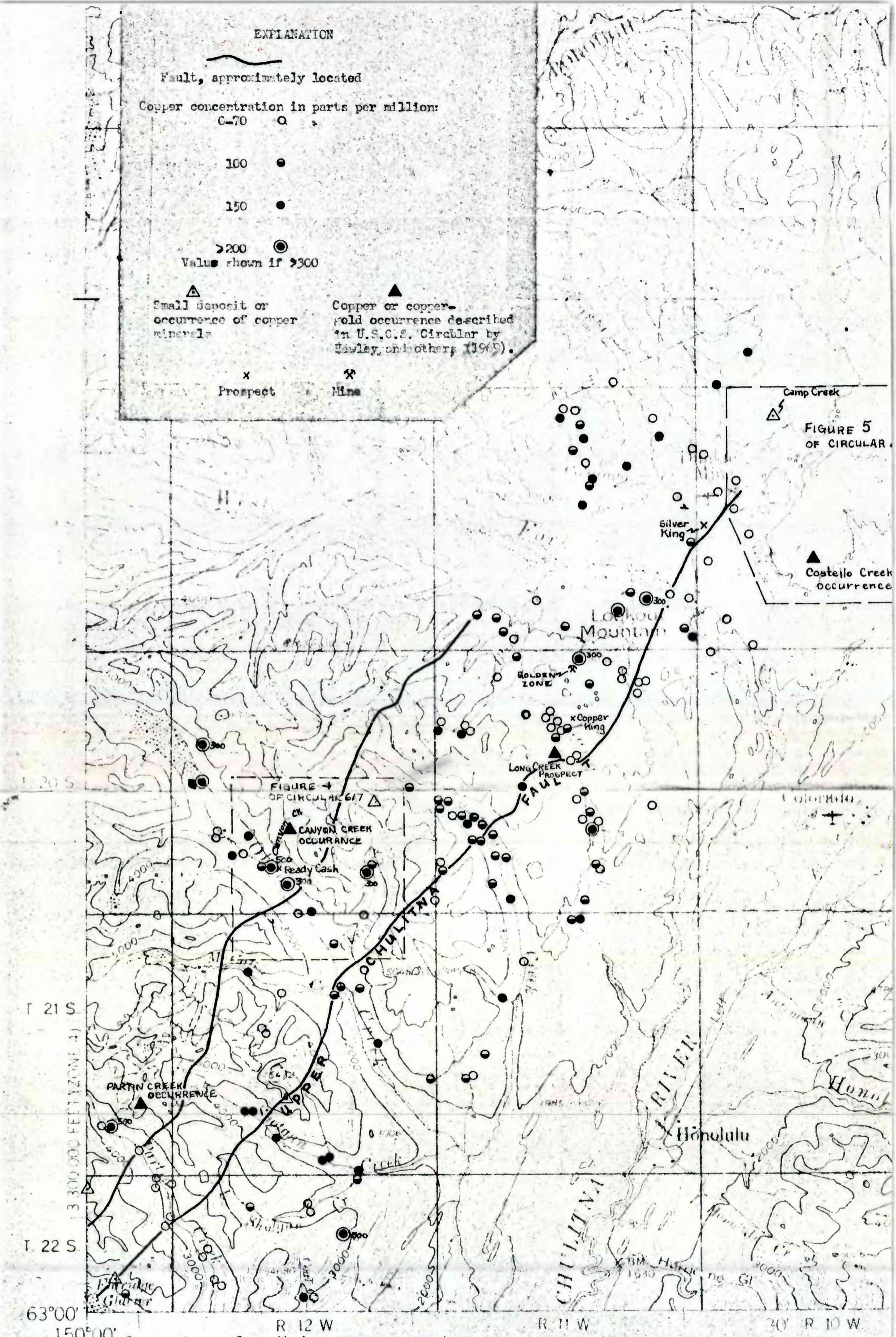
FIGURE 4. -- Copper concentration in stream sediment sampler and location of major faults and copper-bearing deposits.
