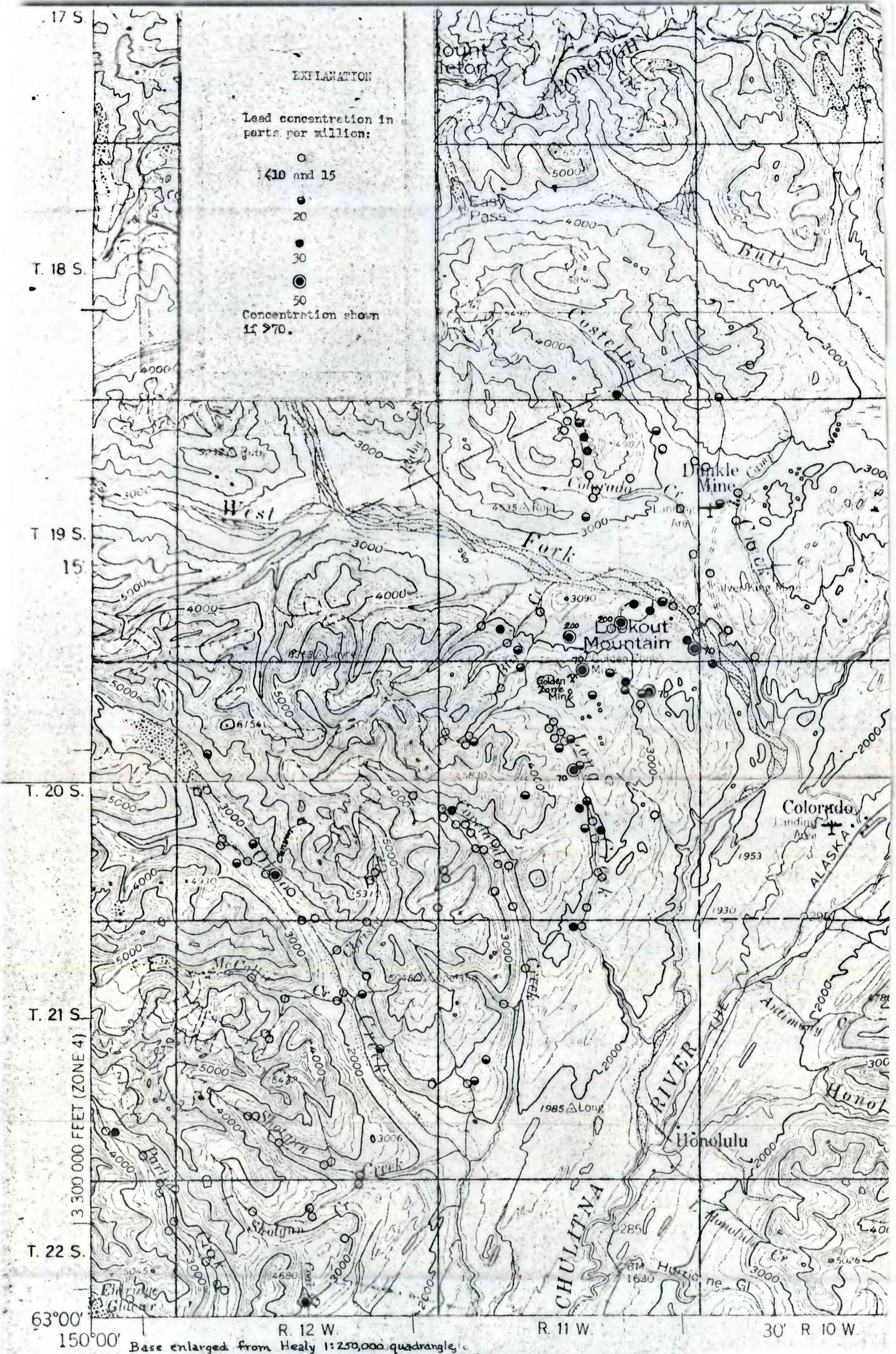
FIGURE 8. --- lead concentration in stream sediment samples.
