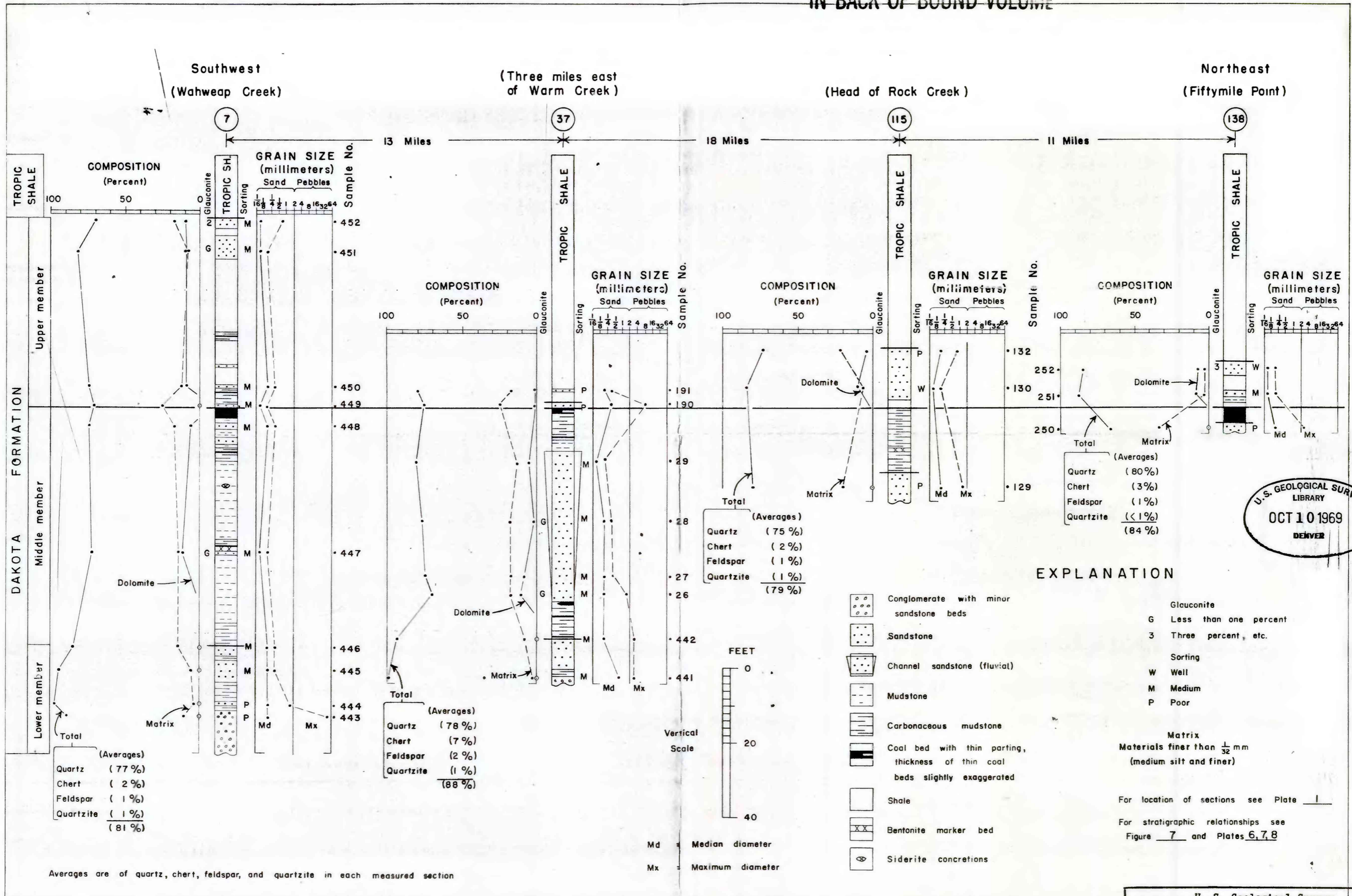
PLATE 2. MINERALOGY OF SANDSTONES IN THE DAKOTA FORMATION
