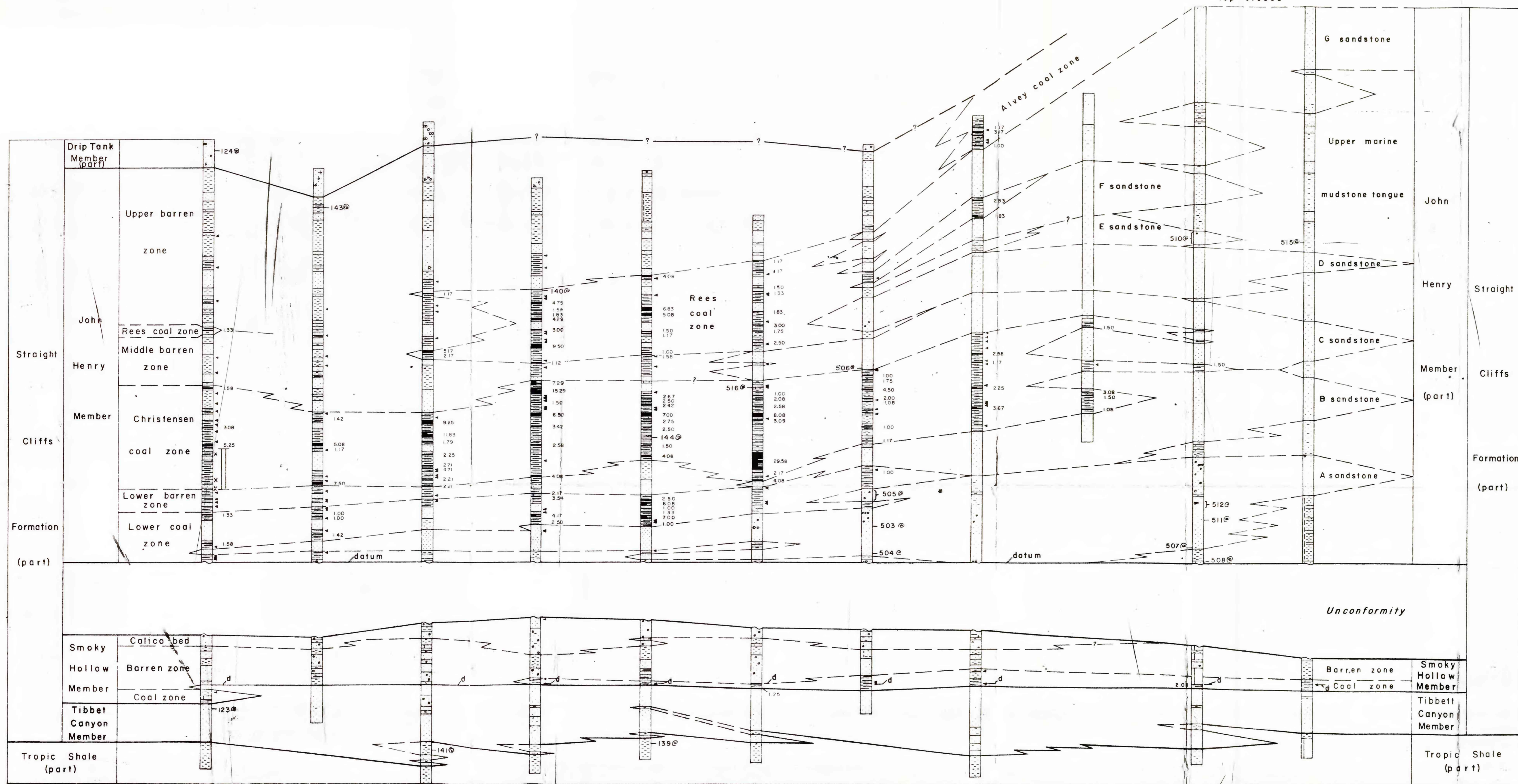
PLATE 10. MEASURED SECTIONS OF STRAIGHT CLIFFS FORMATION IN NORTHEASTERN PART OF SOUTHEASTERN KAIPAROWITS REGION
