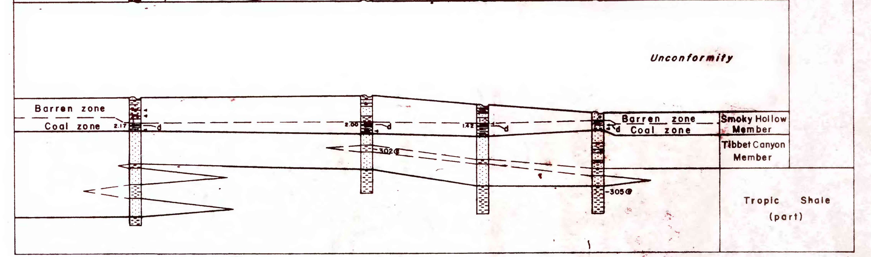
PLATE II. MEASURED SECTIONS OF STRAIGHT CLIFFS FORMATION IN NORTHWESTERN AND EASTERN PARTS OF SOUTHEASTERN KAIPAROWITS REGION
