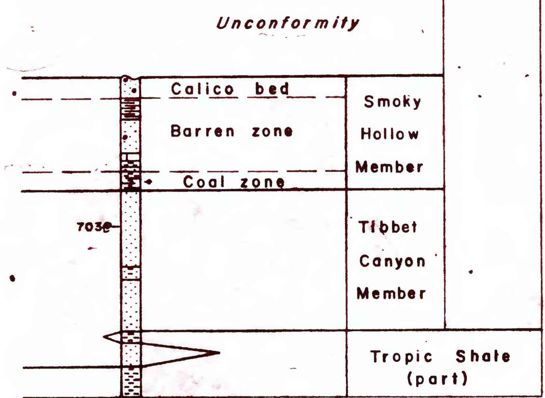
PLATE II. MEASURED SECTIONS OF STRAIGHT CLIFFS FORMATION IN NORTHWESTERN AND EASTERN PARTS OF SOUTHEASTERN KAIPAROWITS REGION
