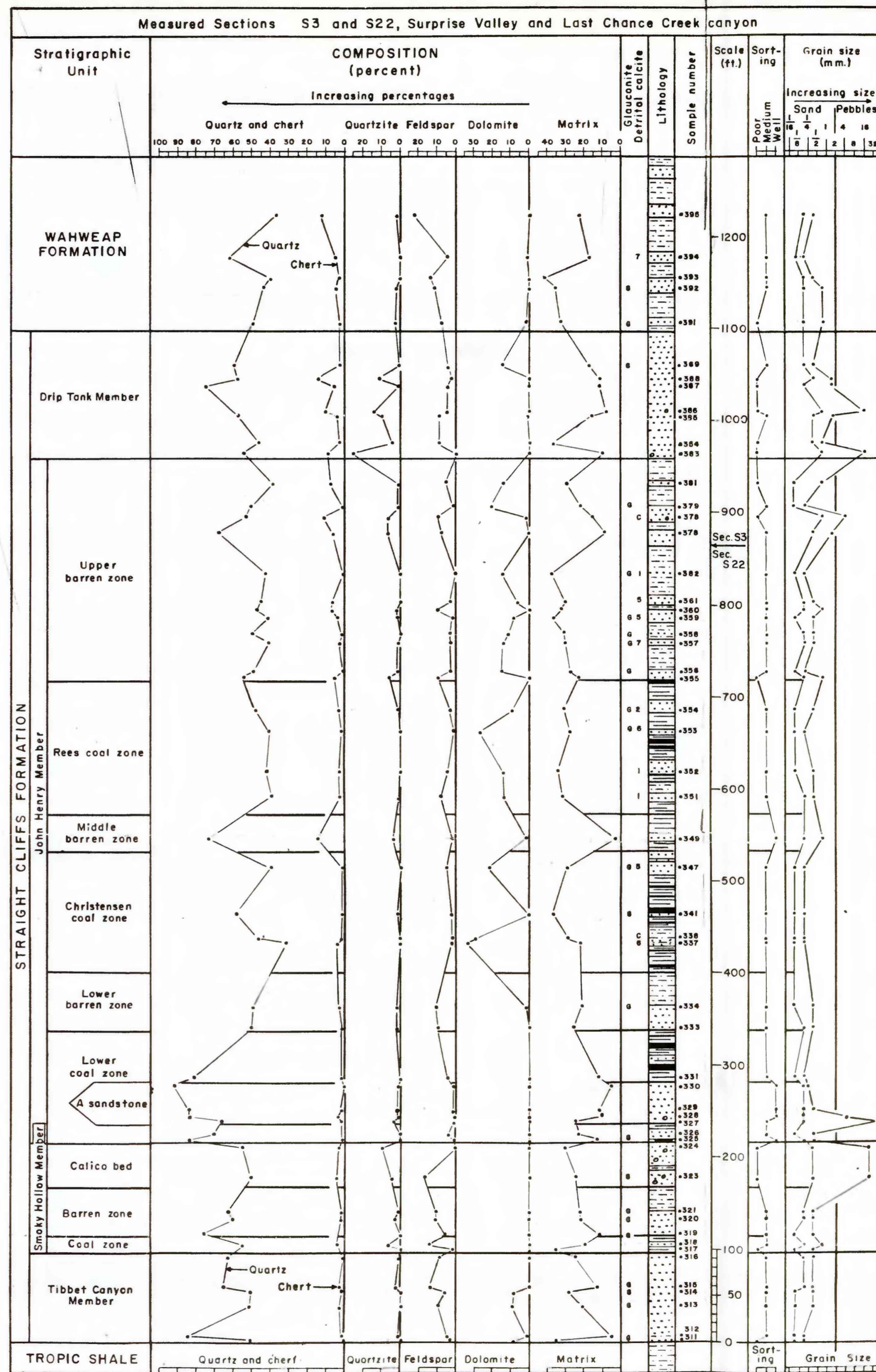
PLATE 12. MINERALOGY OF SANDSTONES IN STRAIGHT CLIFFS FORMATION, SOUTHWESTERN AND CENTRAL PARTS OF SOUTHEASTERN KAIPAROWITS REGION
