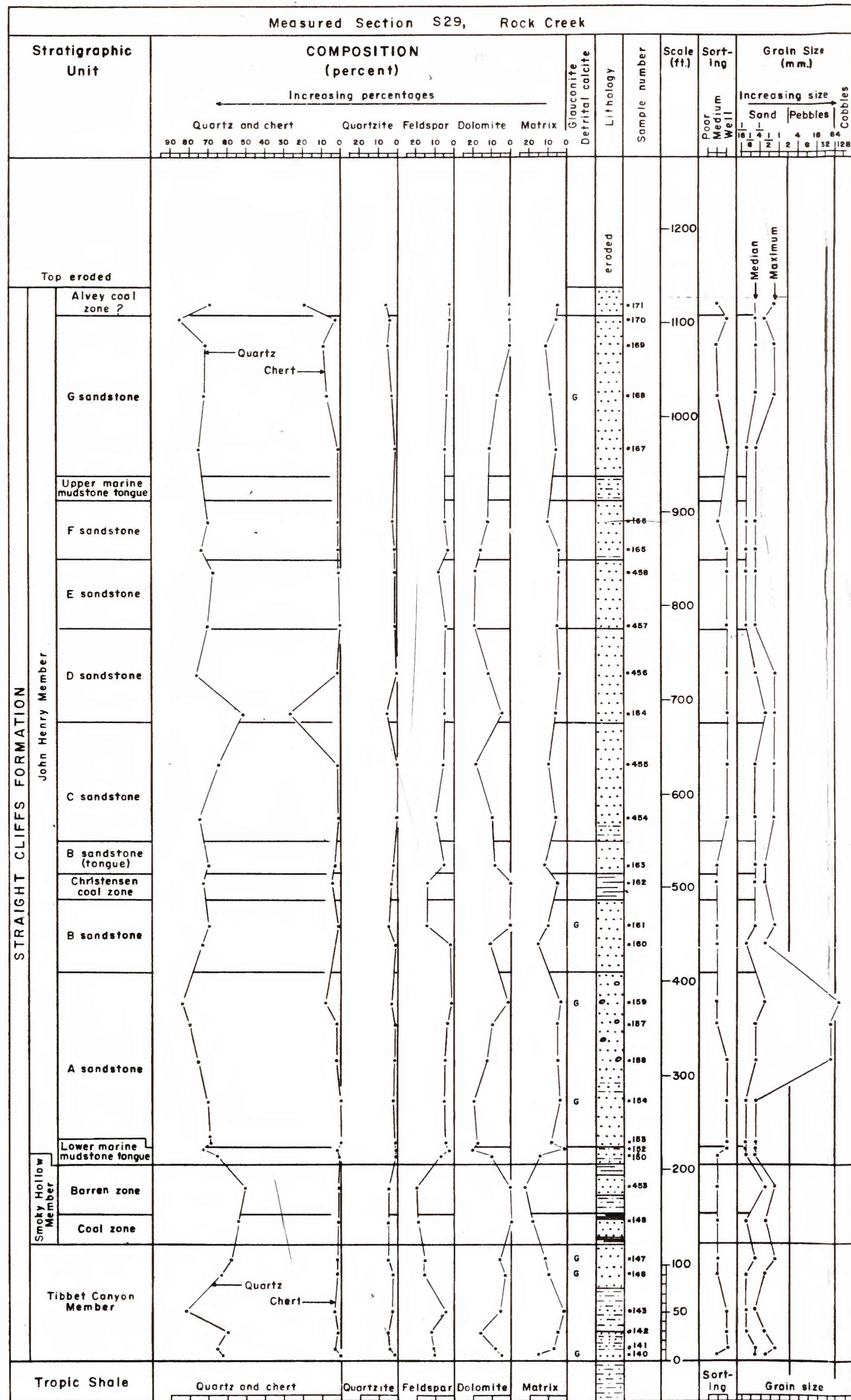
PLATE 13. MINERALOGY OF SANDSTONES IN STRAIGHT CLIFFS FORMATION, EASTERN PART OF SOUTHEASTERN KAIPAROWITS REGION
