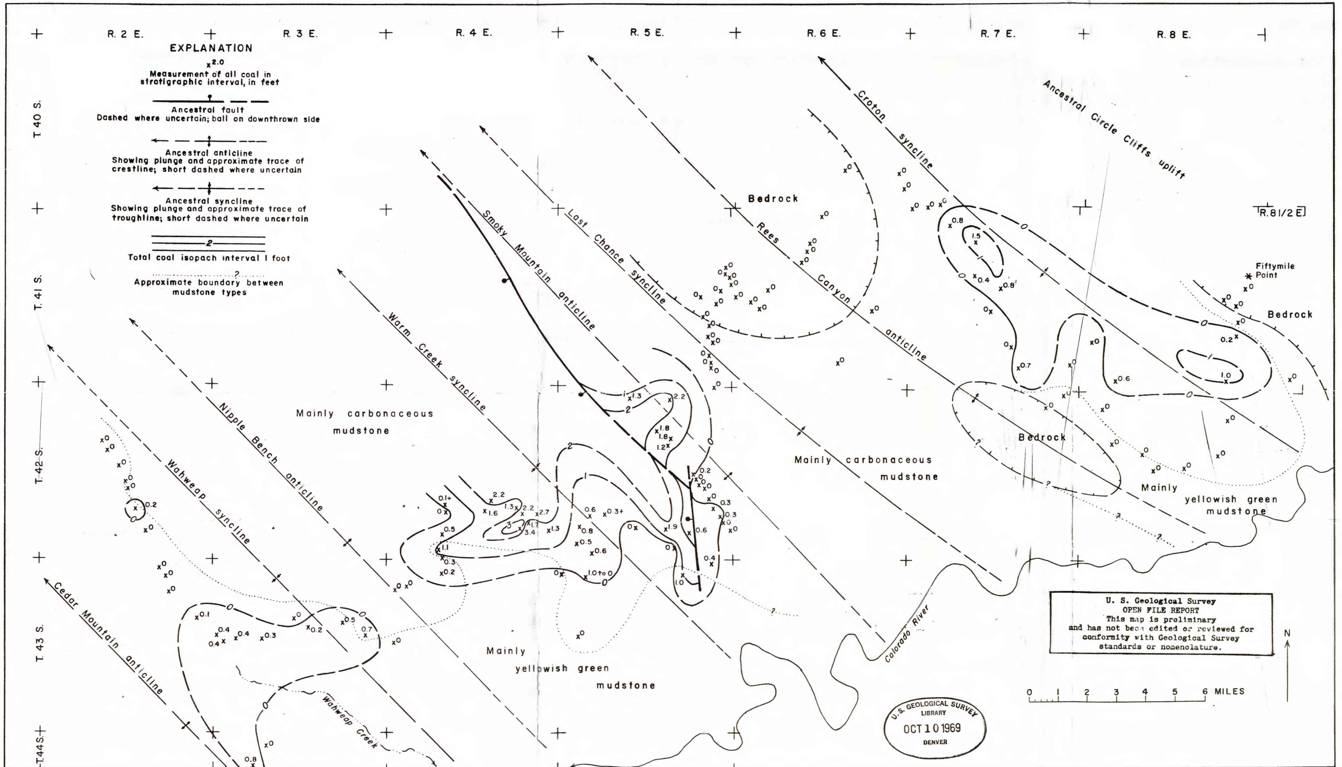
PLATE 14. DISTRIBUTION OF COAL AND MUDSTONE IN MIDDLE MEMBER OF DAKOTA FORMATION BELOW BENTONITE MARKER BED
