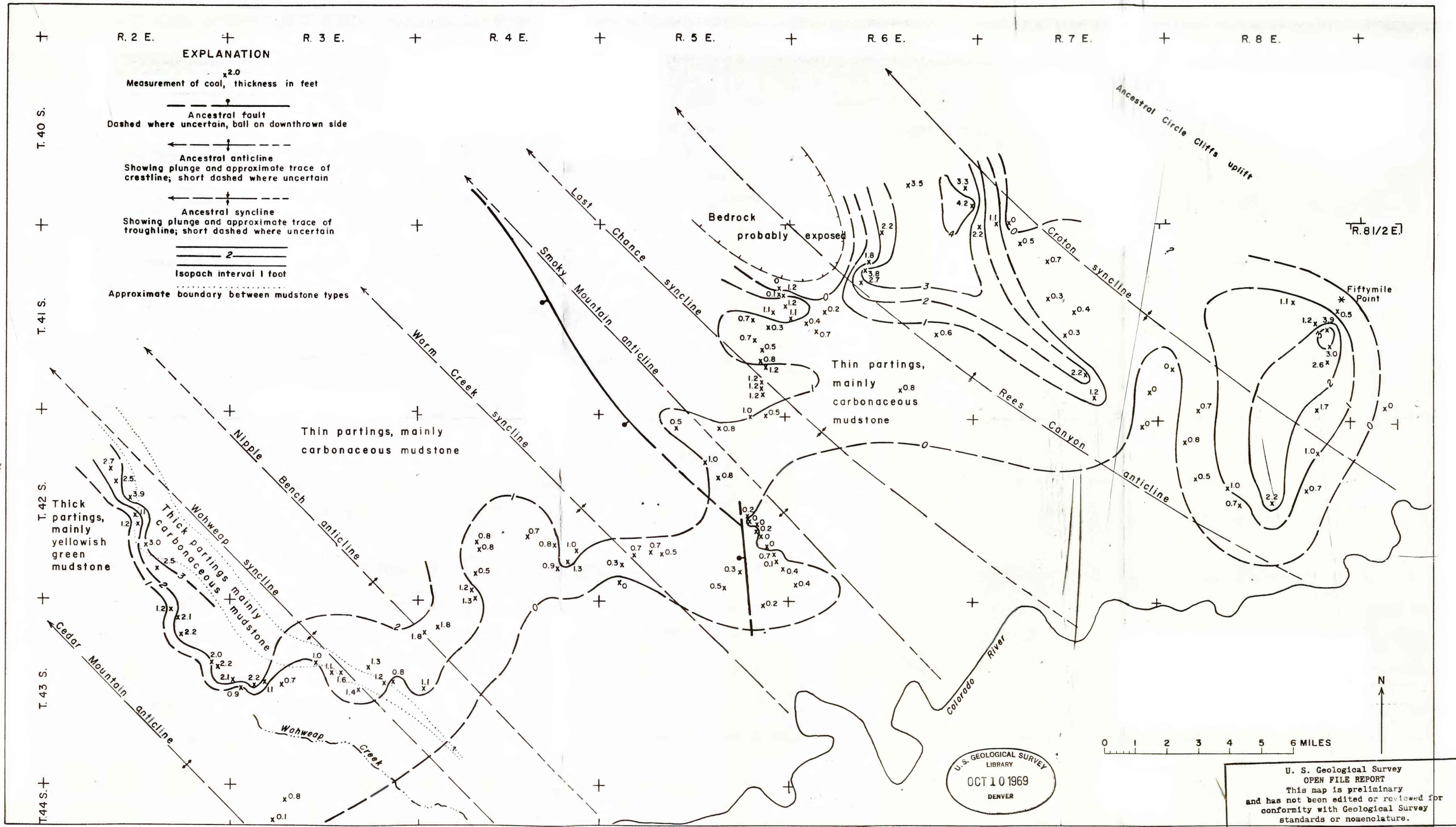
PLATE 16. DISTRIBUTION OF COAL AND PARTINGS IN COAL BED NO. 4, MIDDLE MEMBER OF DAKOTA FORMATION
