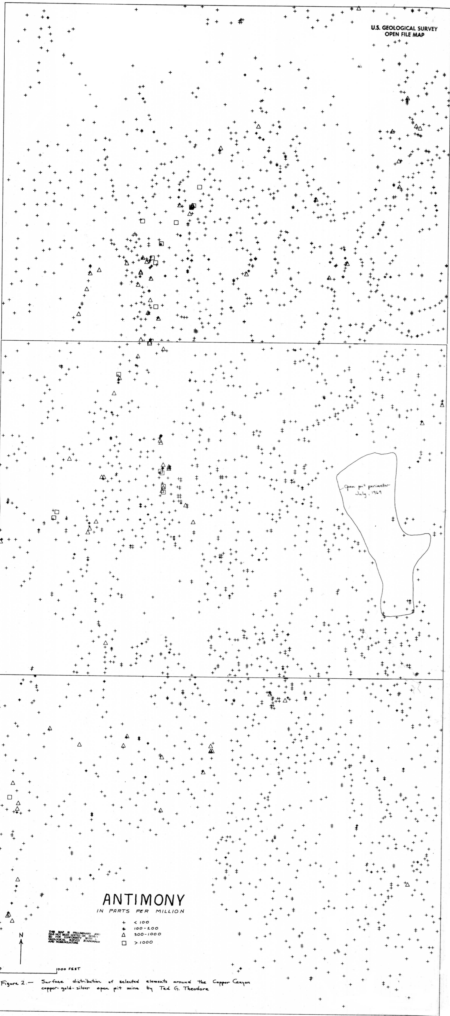
Figure 3.— Surface distribution of selected elements around the Copper Canyon copper-gold-silver open pit mine by Ted G. Theodore
