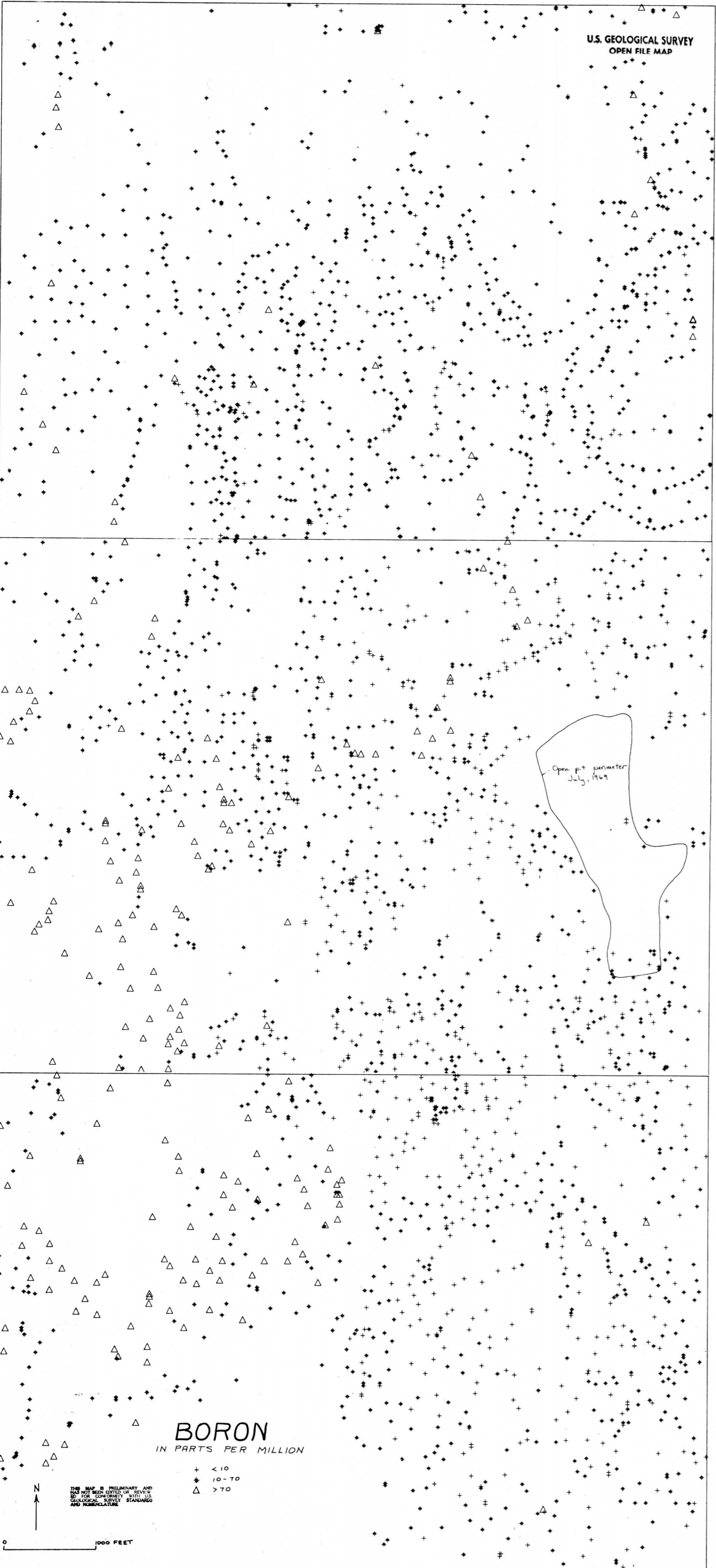
Figure 6. - Surface distribution of selected elements around the Copper Canyon copper-gold-silver open-pit mine by Ted G. Theodore
