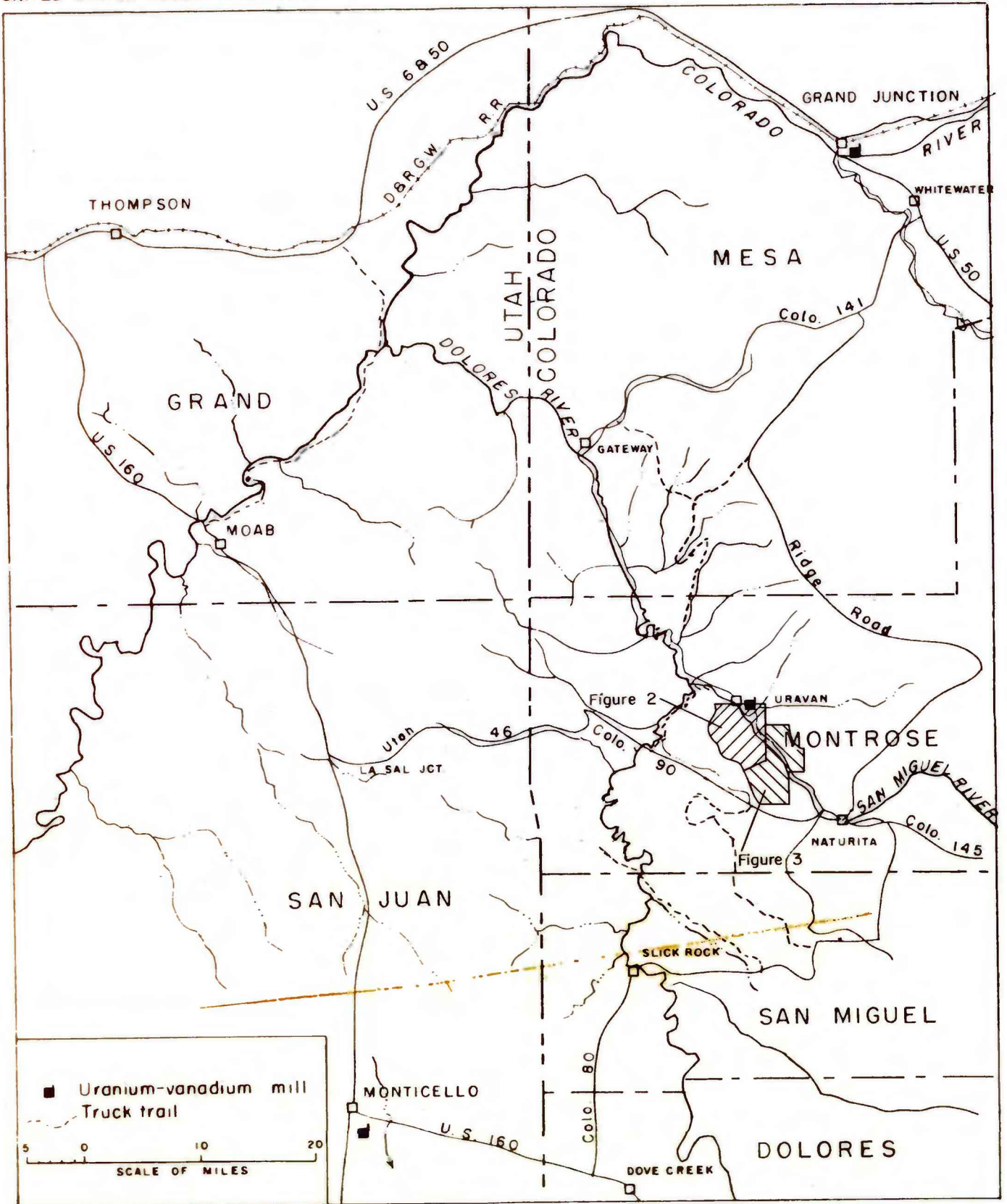
Figure 1.--INDEX MAP OF PART OF THE COLORADO PLATEAU SHOWING LOCATION OF FIGURES 2 AND 3 IN THE URAVAN DISTRICT, MONTROSE COUNTY, COLORADO
