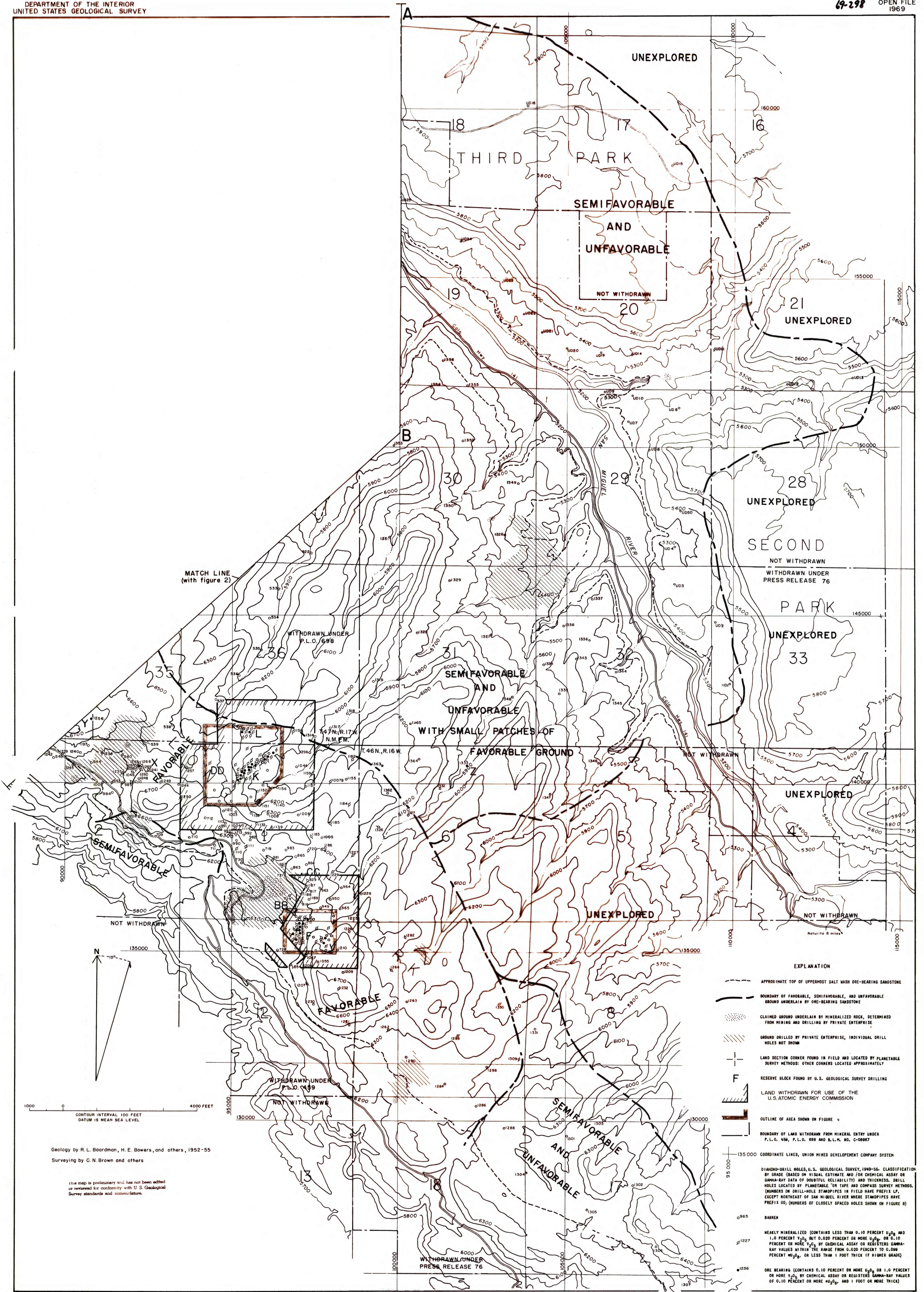
Figure 3.--MAP OF THE SOUTHEASTERN PART OF THE URAVAN DISTRICT, MONTROSE COUNTY, COLO.
