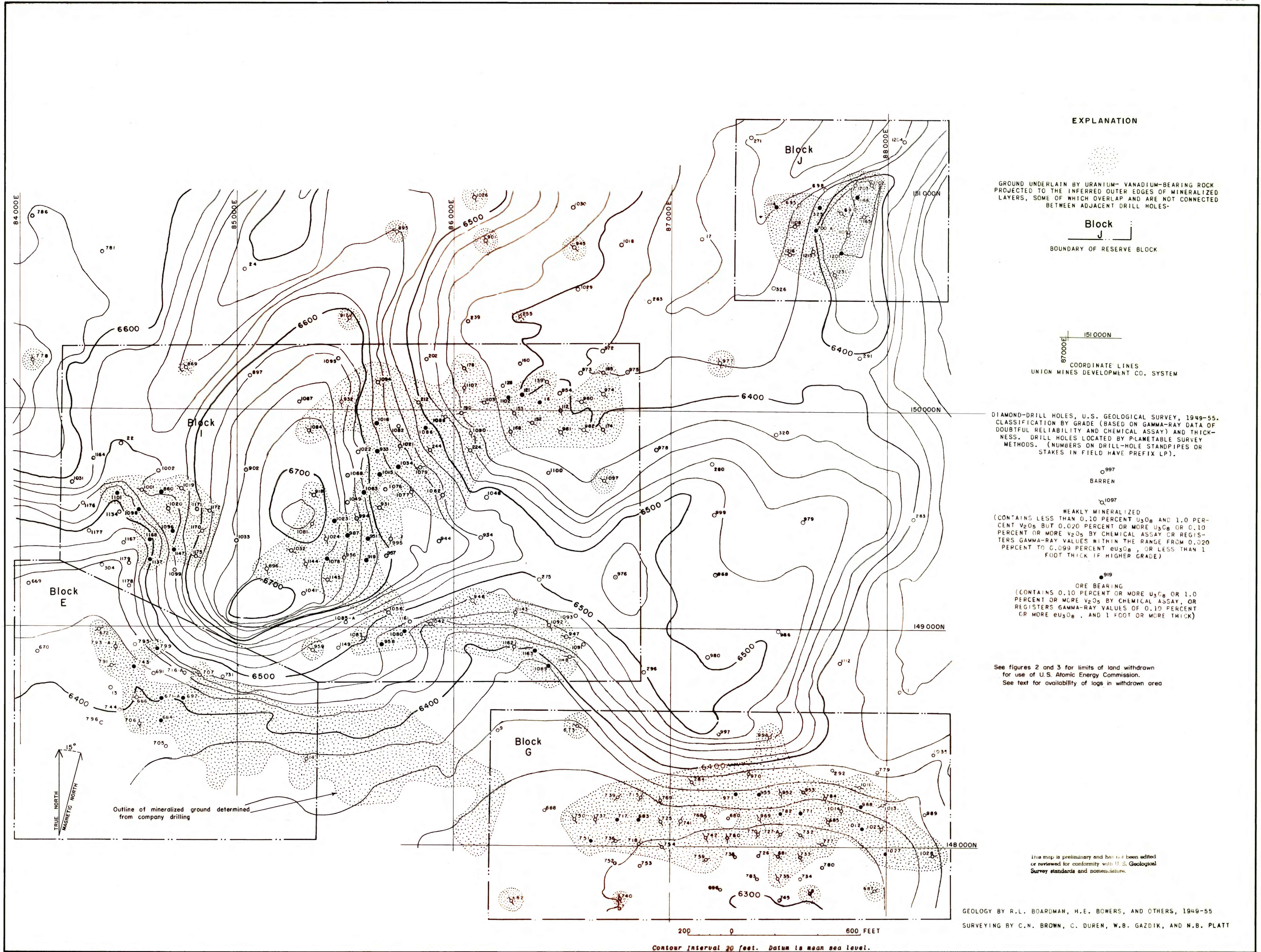
Figure 7.-- MAP OF PART OF EAST-CENTRAL LONG PARK, URAVAN DISTRICT, MONTROSE COUNTY, COLORADO
