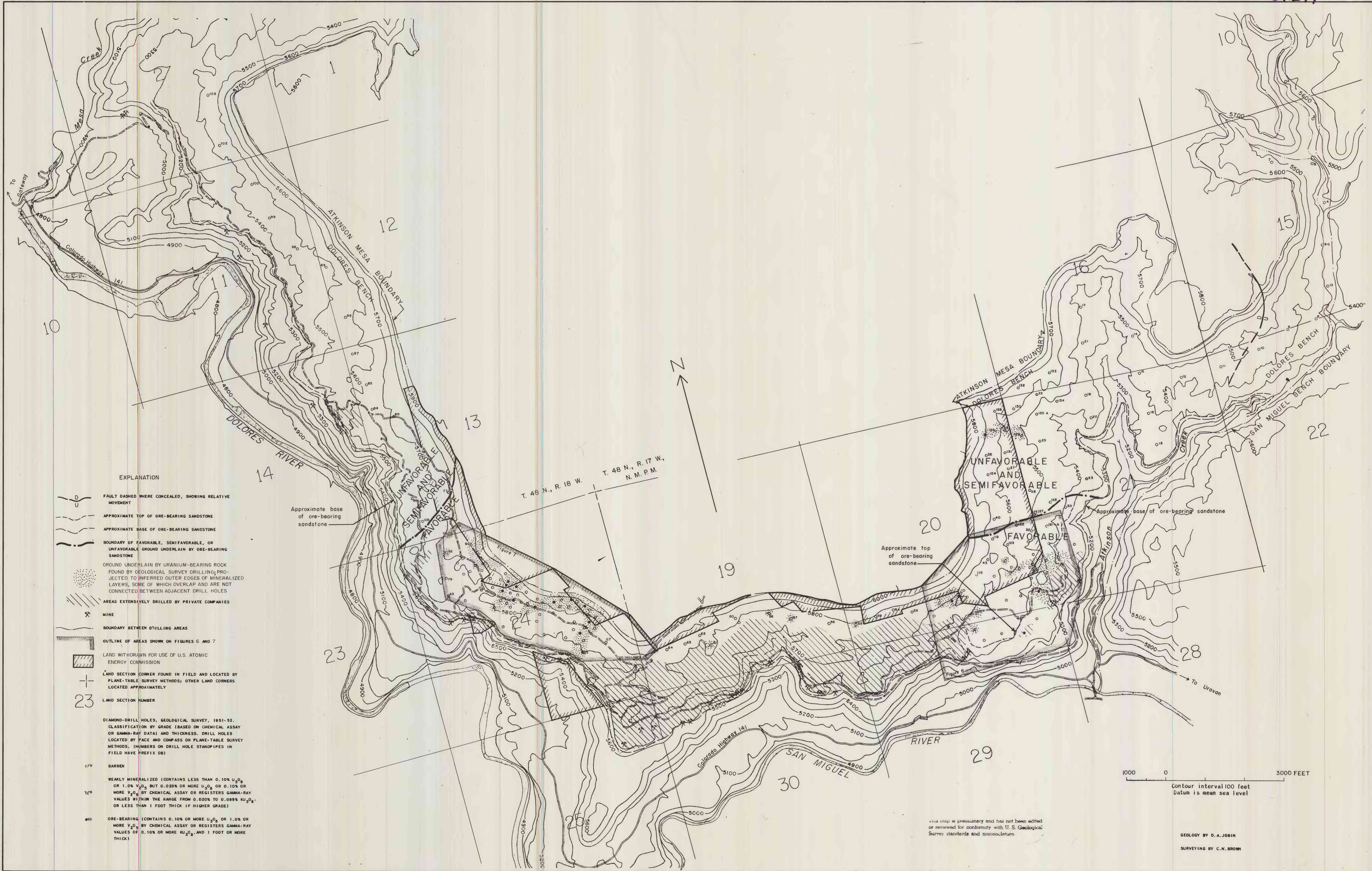
FIGURE 3.--MAP OF THE DOLORES BENCH AREA, MONTROSE COUNTY, COLORADO
