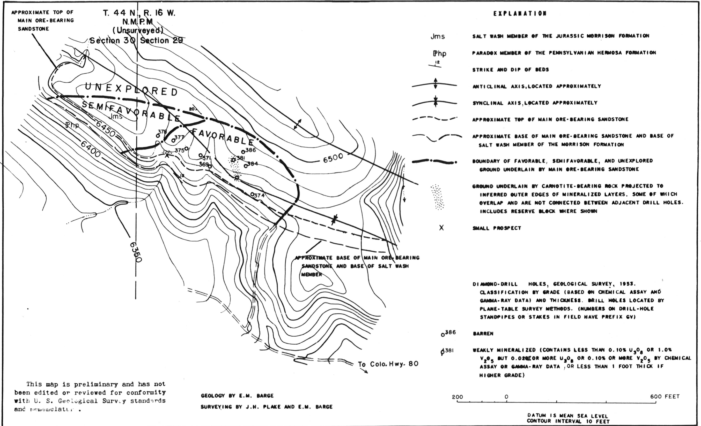
Figure 17.-- MAP SHOWING LOCATION OF HOLES DRILLED BY GEOLOGICAL SURVEY IN THE SUNSET CLAIM, GYPSUM VALLEY DISTRICT, SAN MIGUEL COUNTY, COLORADO
