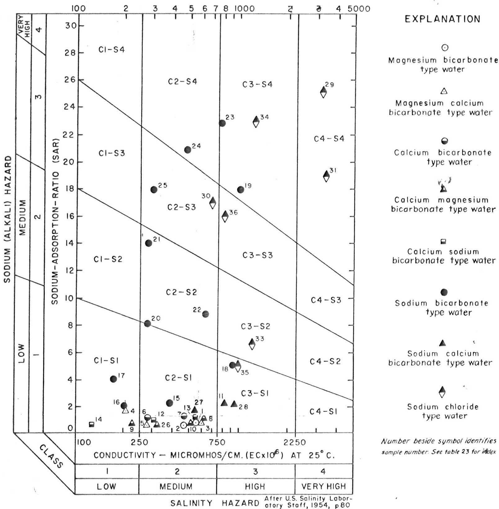
FIGURE 37.— Diagram showing the classification of the most widely distributed chemical types of ground water for irrigation in the Fresno area.
