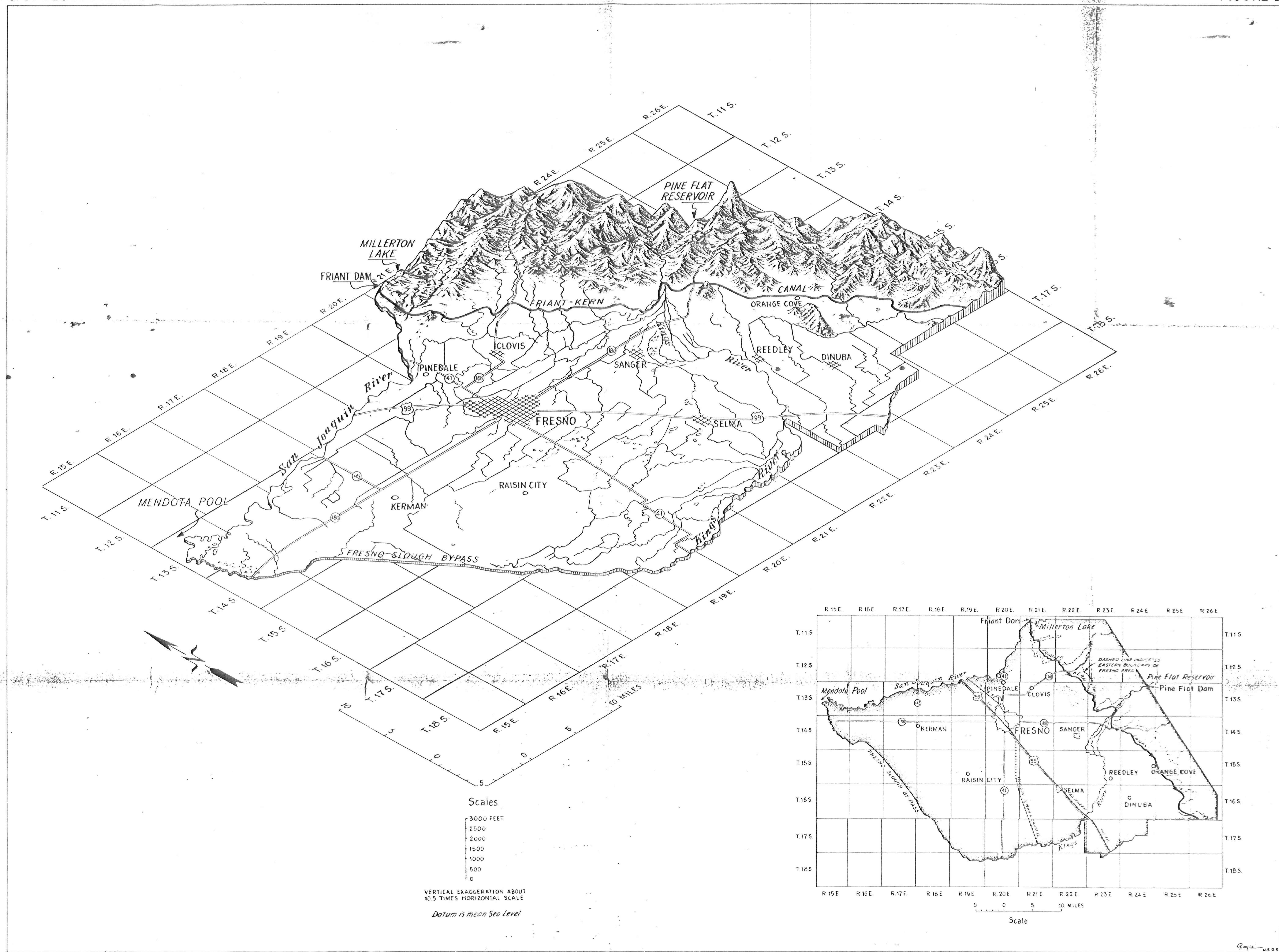
FIGURE 2. ISOMETRIC BLOCK DIAGRAM OF THE FRESNO AREA, SAN JOAQUIN VALLEY, CALIFORNIA
