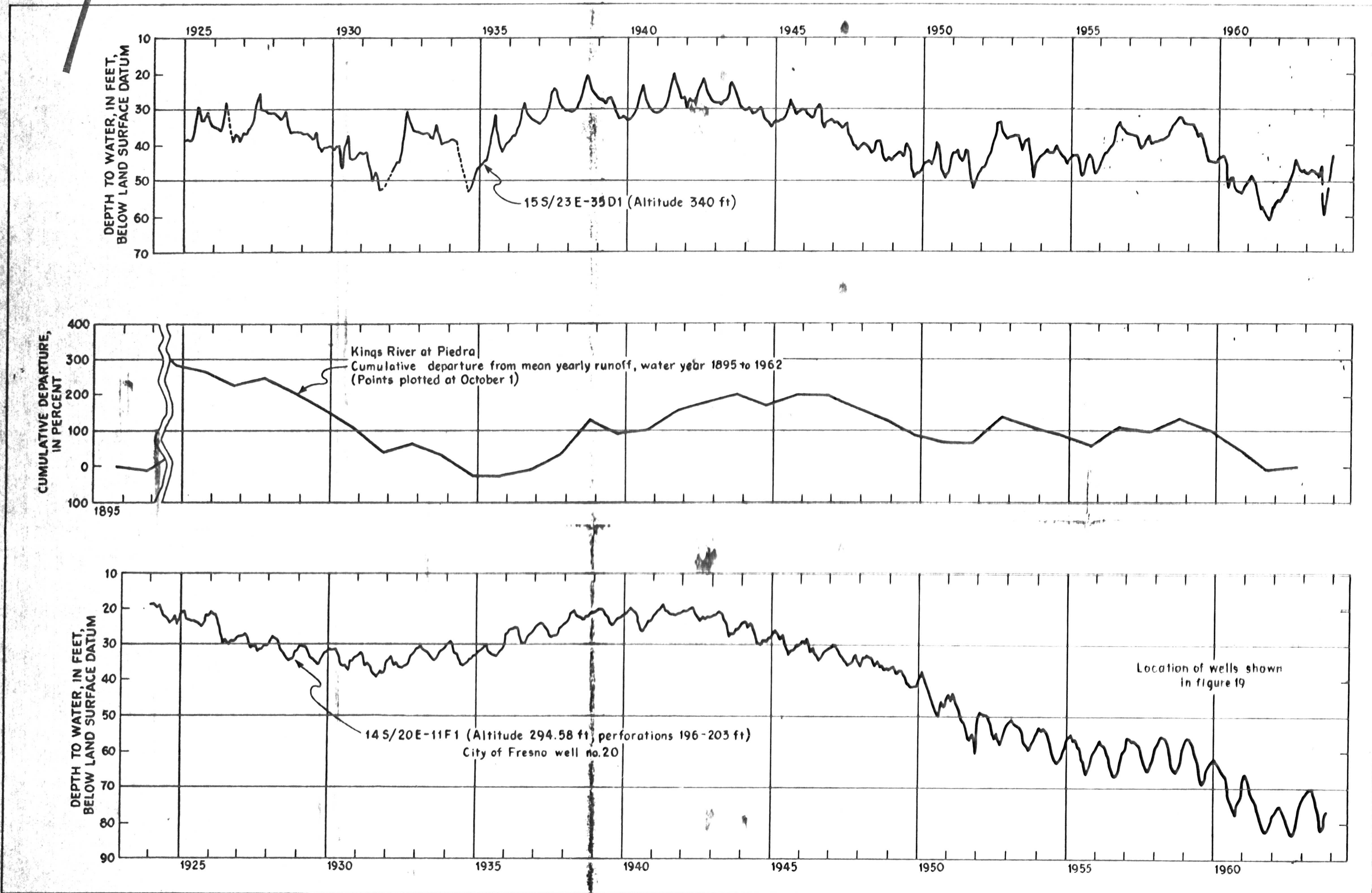
FIGURE 23.—HYDROGRAPHS SHOWING RELATION OF WATER-LEVEL FLUCTUATIONS IN TWO WELLS TO CUMULATIVE DEPARTURE FROM MEAN YEARLY RUNOFF IN KINGS RIVER, FRESNO AREA, SAN JOAQUIN VALLEY, CALIFORNIA
