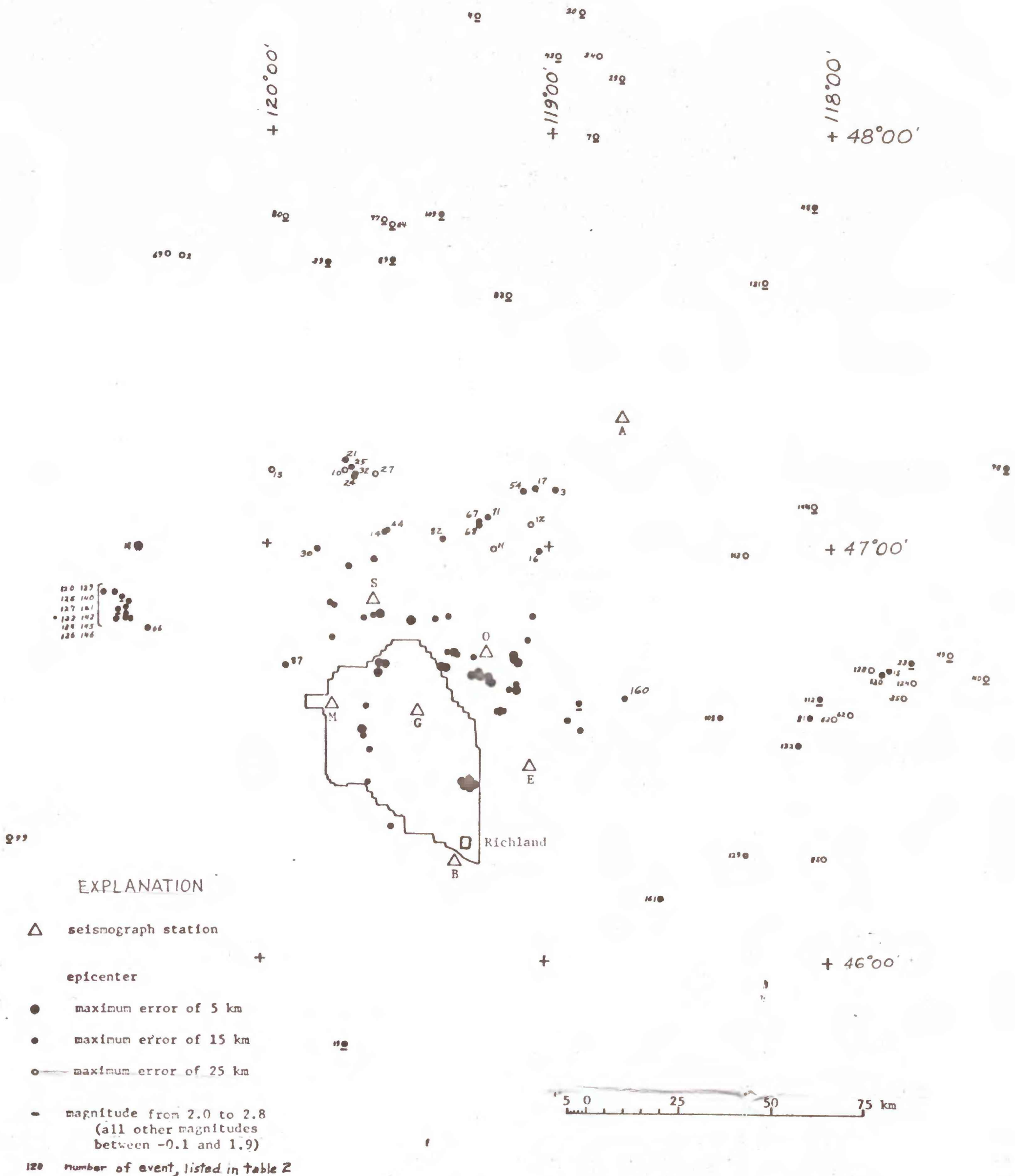
FIGURE 25.—Locations of epicenters of seismic events occurring in south-central Washington, March 23-December 31, 1969. (Also see fig. 4.)
