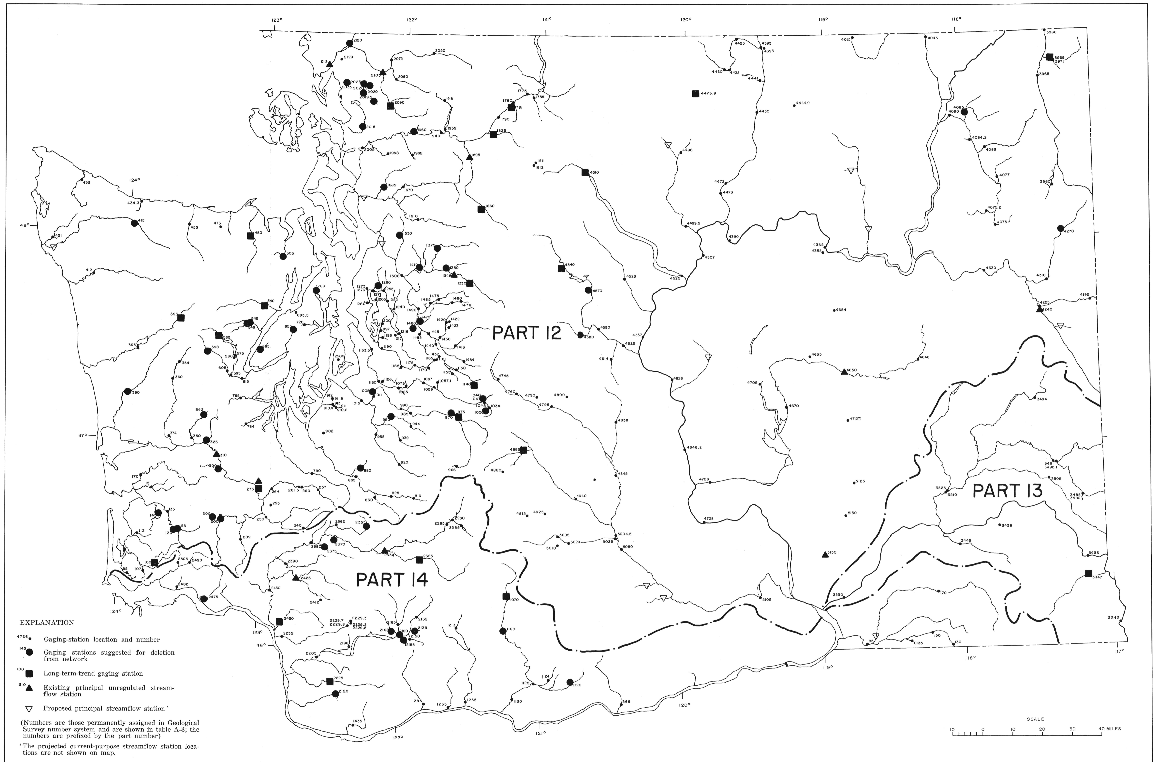
FIGURE 5.—Locations of gaging stations for continuance, addition and deletion in the existing network.
