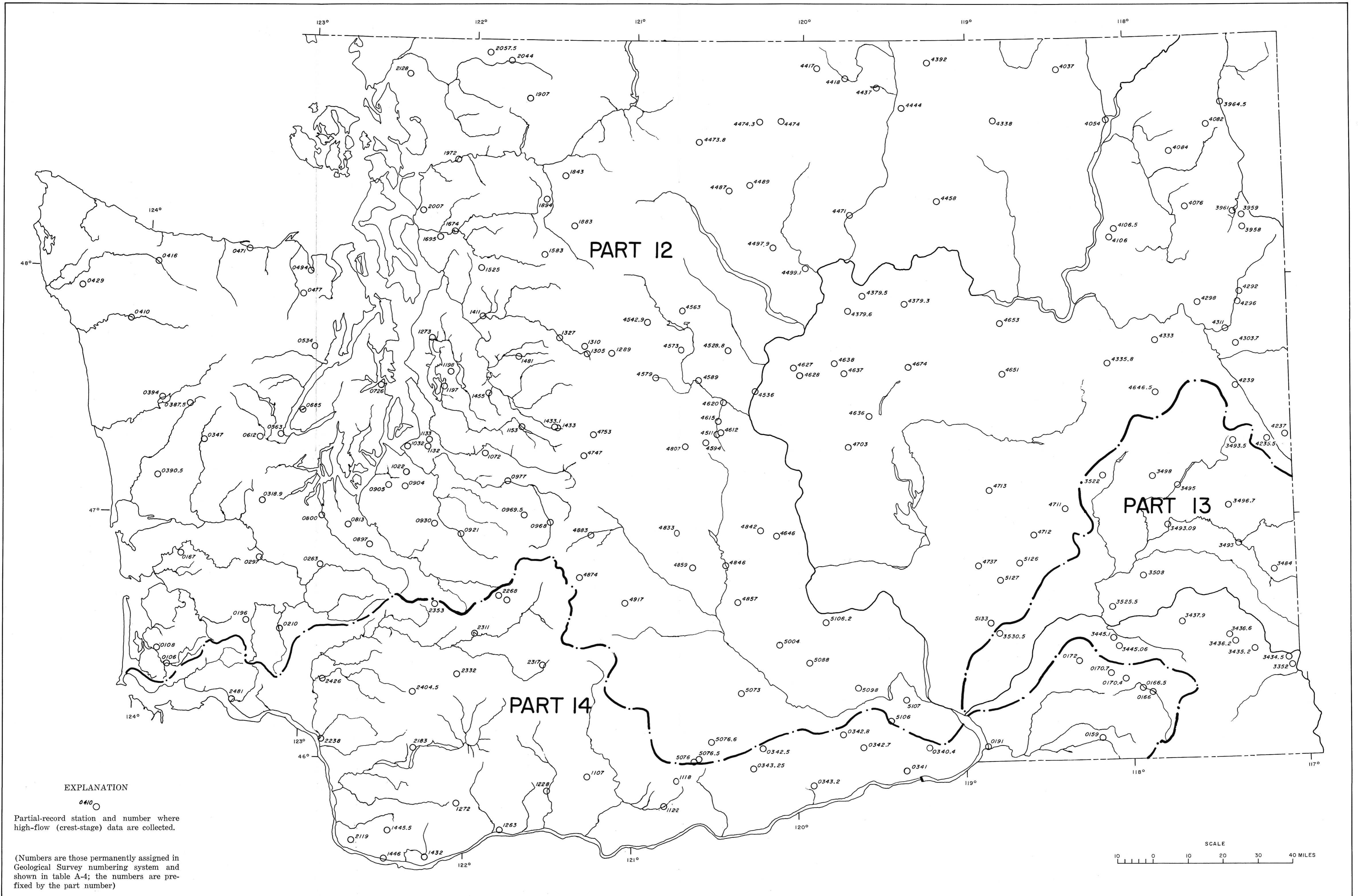
FIGURE 6.—Locations of partial-record stations where high-flow data are being collected.
