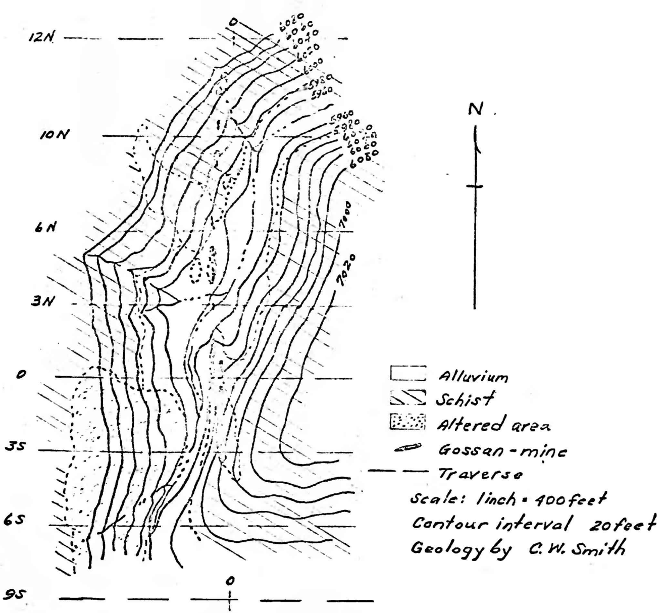
GENERALIZED GEOLOGIC MAP AND EM TRAVERSES MINDAHA MINE AREA
