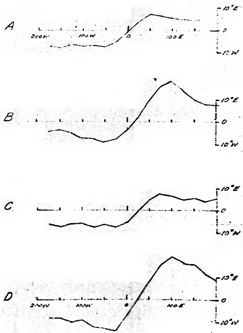
FIGURE 4. DIP-ANGLE PROFILES, WADI FIG PROSPECTS.
