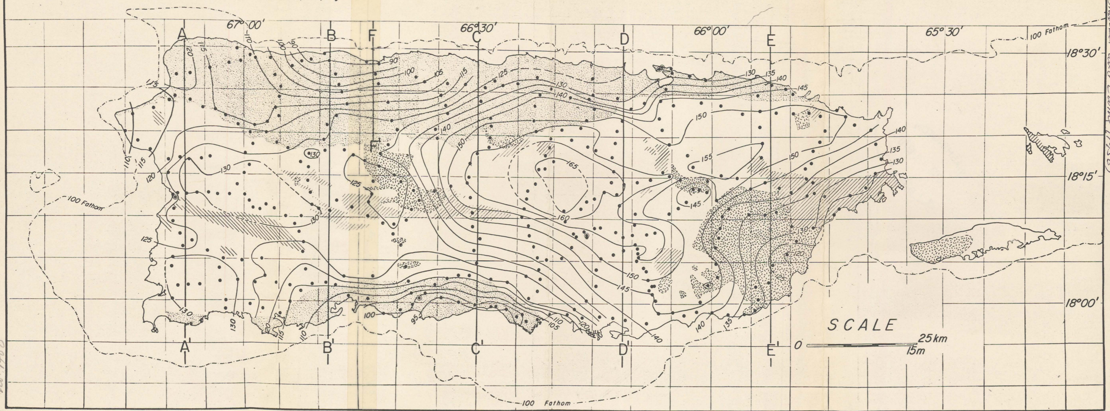
CONTOURED MODIFIED BOUGUER ANOMALIES AND SURFACE GEOLOGIC FORMATIONS IN PUERTO RICO
