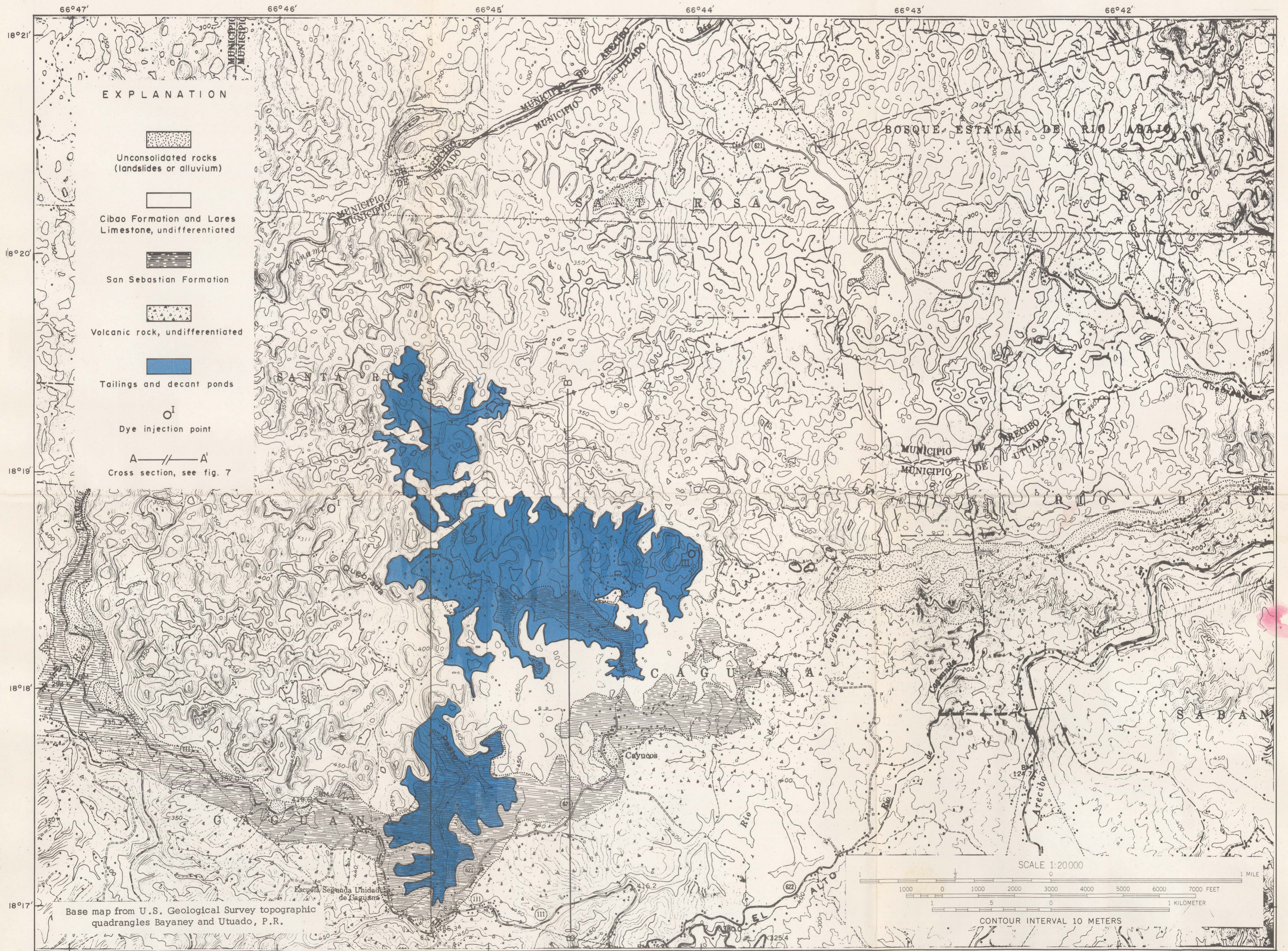
Figure 2.--Generalized geology of tailings disposal area.
