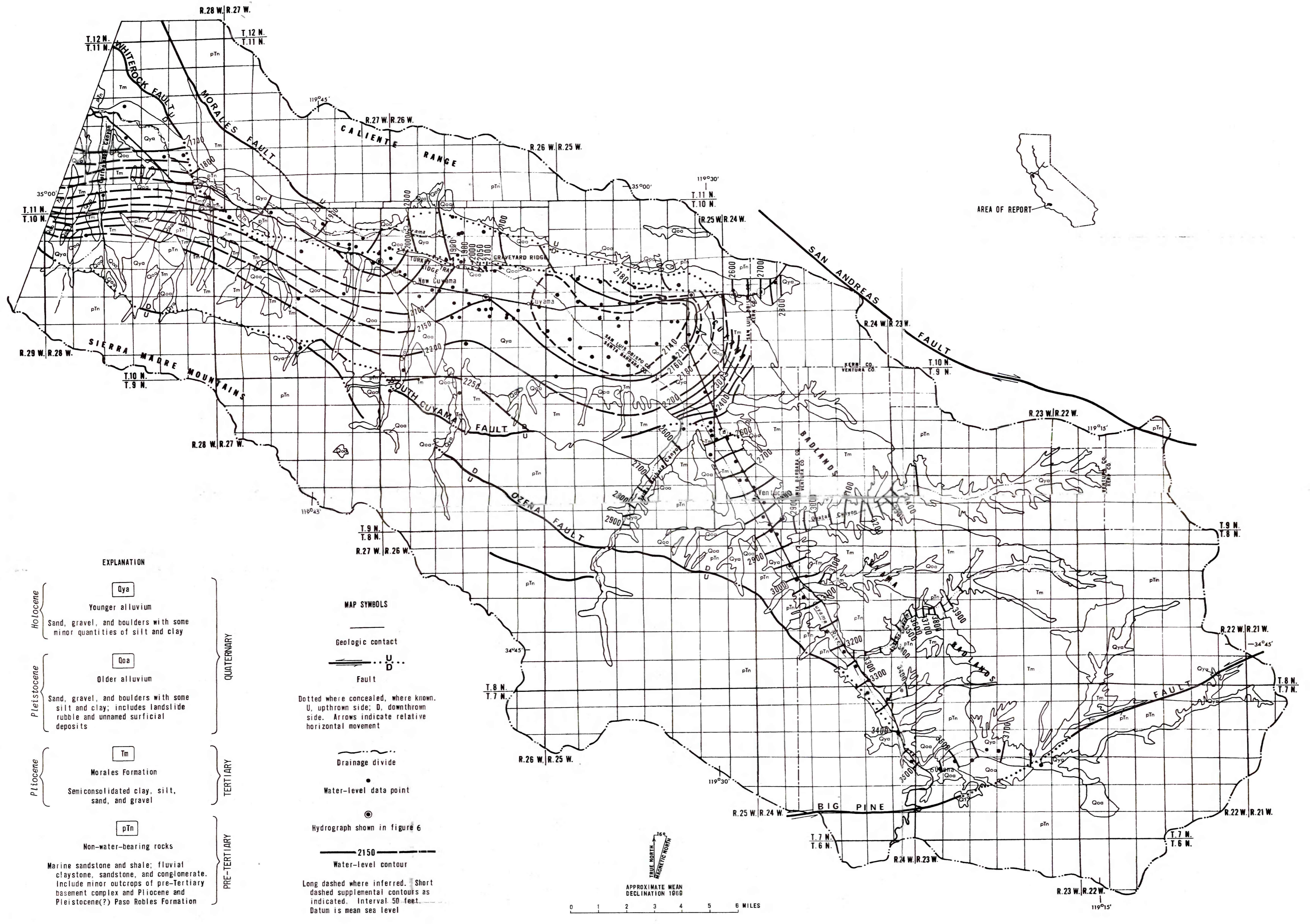
MAP OF CUYAMA VALLEY, CALIFORNIA, SHOWING WATER-LEVEL CONTOURS FOR SUMMER 1966
