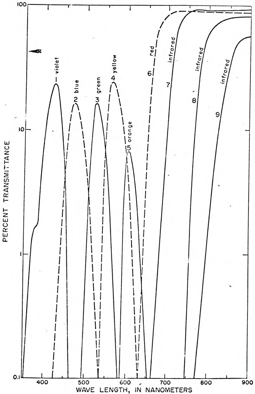
Figure 8.--Nominal transmission curves for multiband filters used with ITEK 9-lens camera. Numbers identify frames described in text. Data from NASA.
