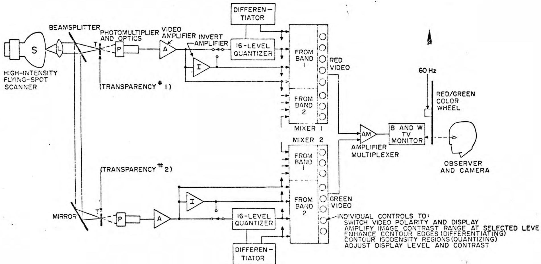
Figure 2.--Generalized diagram of electronic image enhancement system. Modified from data furnished by Philco-Ford Corporation.
