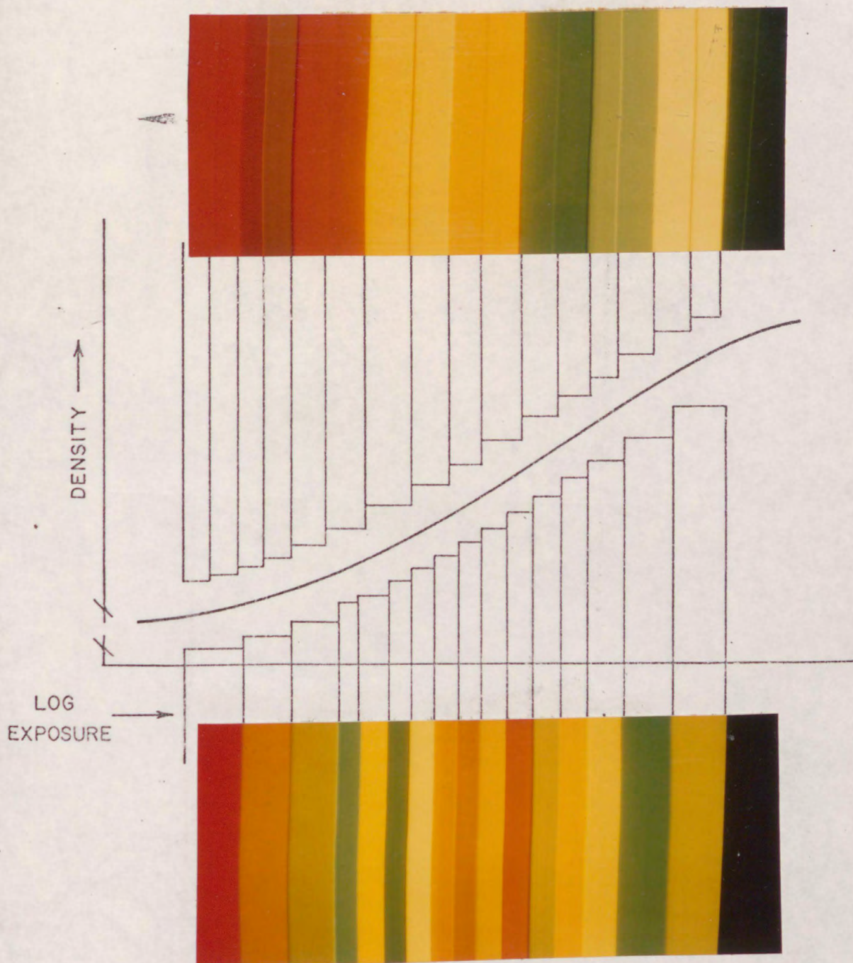
Figure 3.--Diagram illustrating 16-level quantizing of image density curve. Color photographs were taken by means of an internally generated ramp waveform which determines position, width, and color of the density levels or slices. Upper photograph illustrates subequal spacing of slices throughout the density range. Lower photograph illustrates how the spacing can be made nonlinear, to fit nonlinear parts of the density curve.
