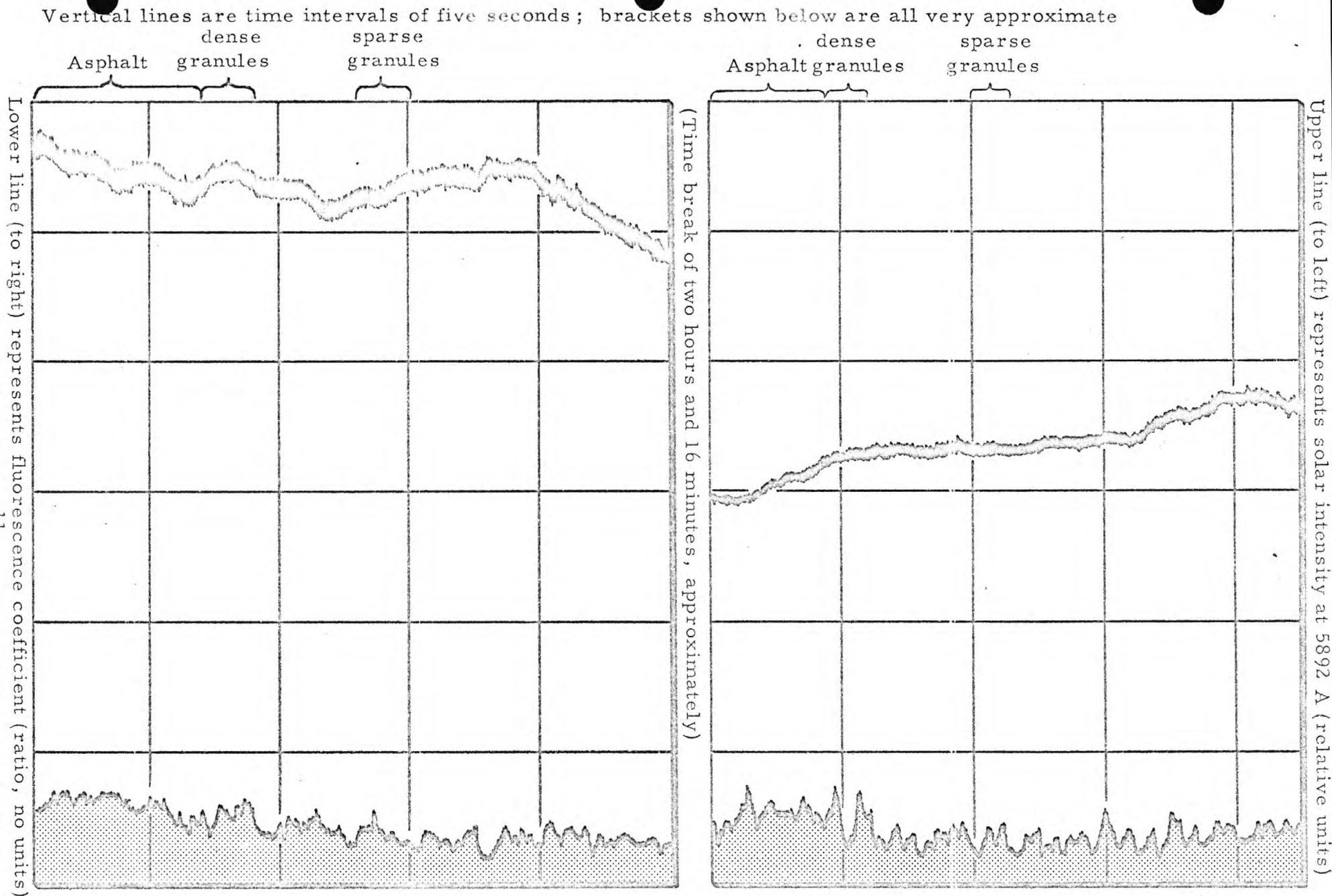
Figure 4. FLD response during airborne traverses over two swaths of fluorescent granules scattered on barren ground (December 6, 10:13 am and 12:29 pm Mountain Standard Time, Needles, Calif.)
