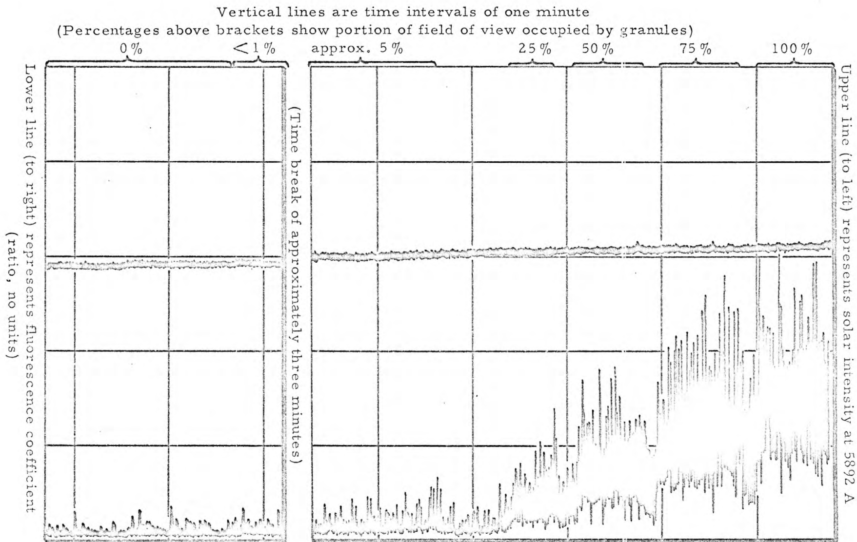
Figure 3. FLD response to varying distributions of fluorescent granules stained with 1.0 % Rhodamine WT (Dec. 4, 4:05 to 4:16 pm Mountain Standard Time, Needles, Calif.)
