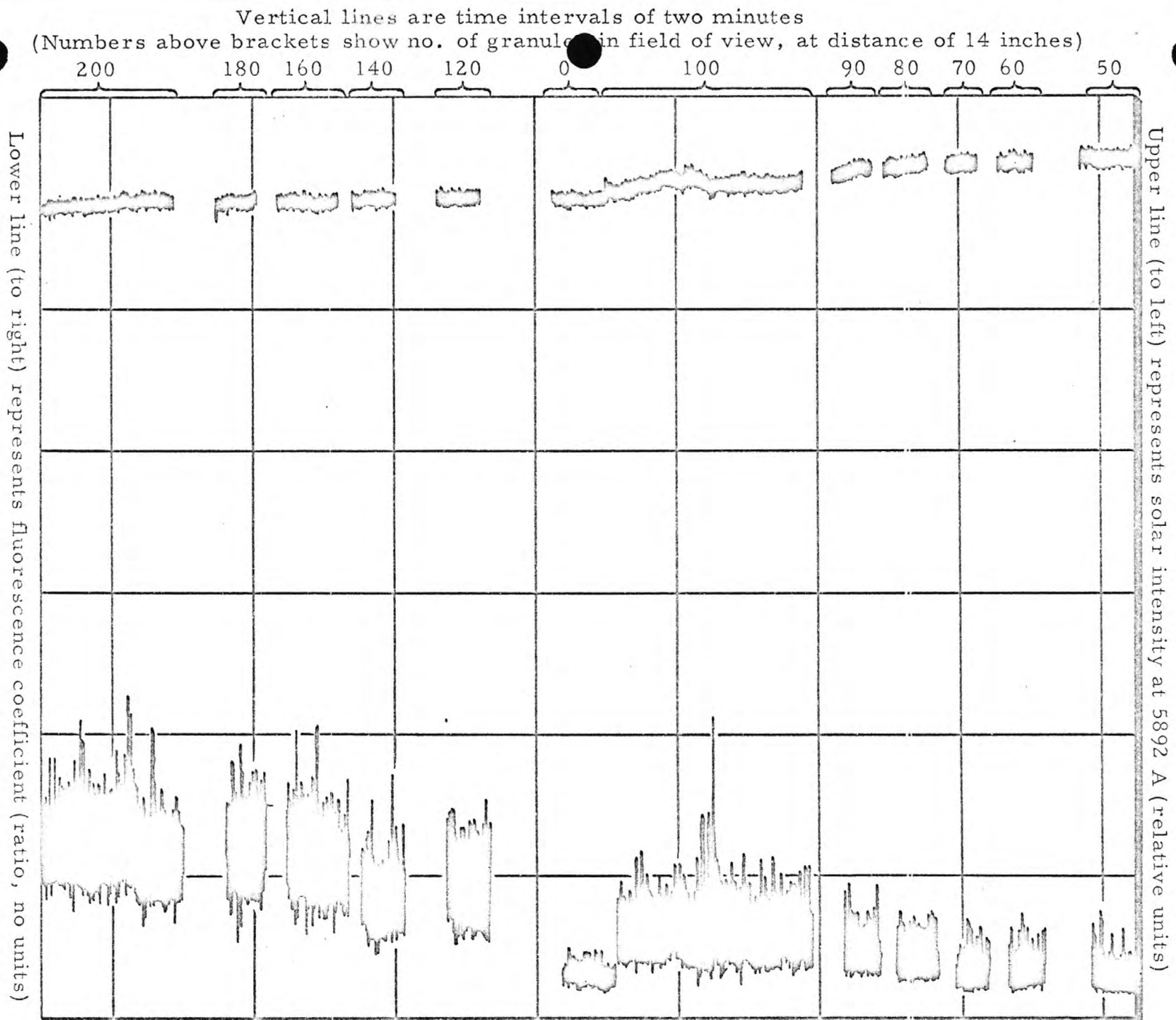
Figure 7. FLD response to fluorescent granules stained with 1.0 % Rhodamine WT, from 50 to 200 granules per 1.3 square inches (Dec. 16, 1:34 to 1:50 pm Pac. Std. Time, Menlo Park, Cal.)
