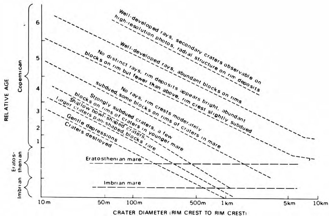
Figure 2.--Relationships between crater morphologies, crater diameters, and postulated ages.
