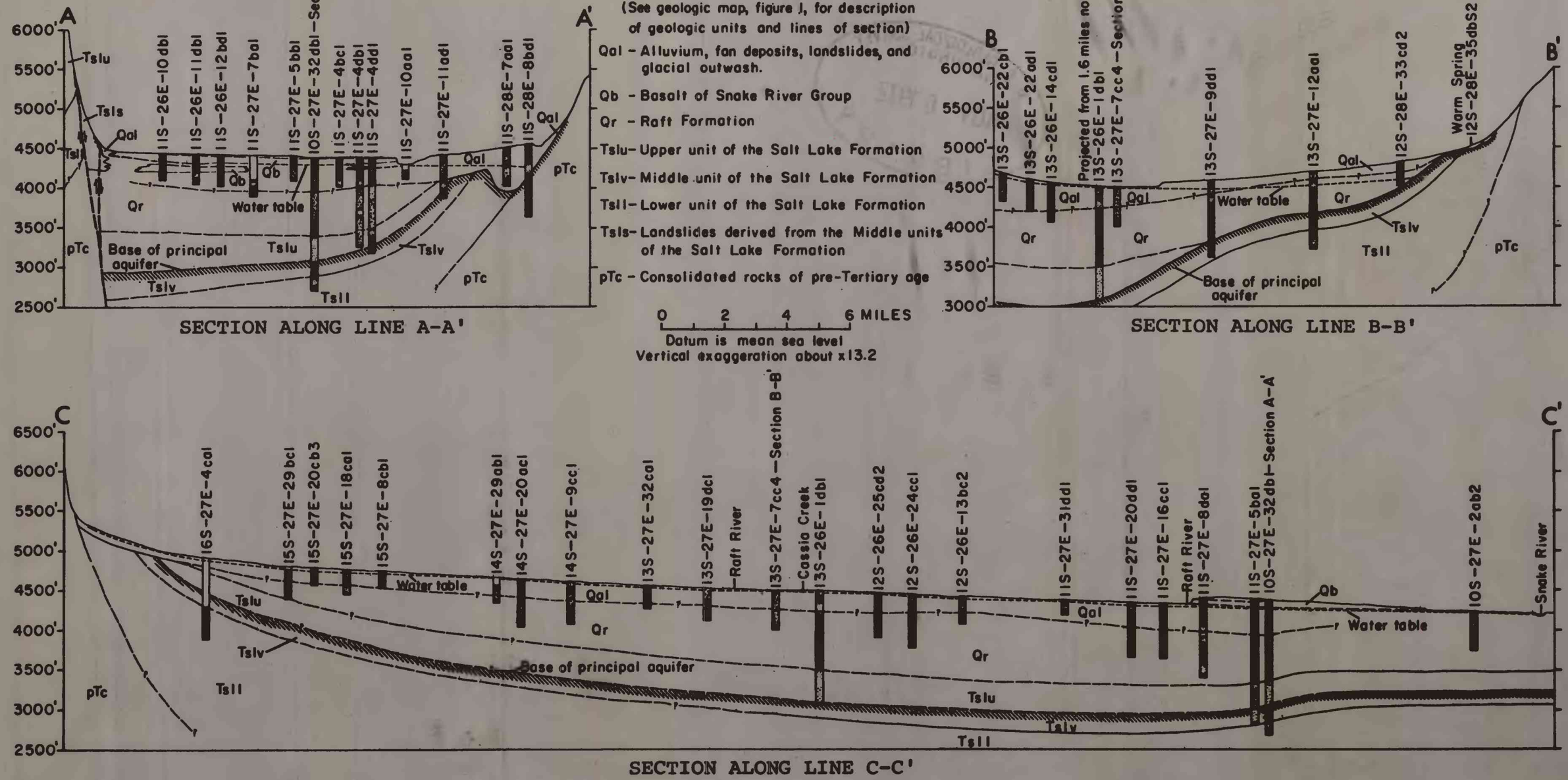
FIGURE 7.--Geologic sections Raft River valley, Idaho.
