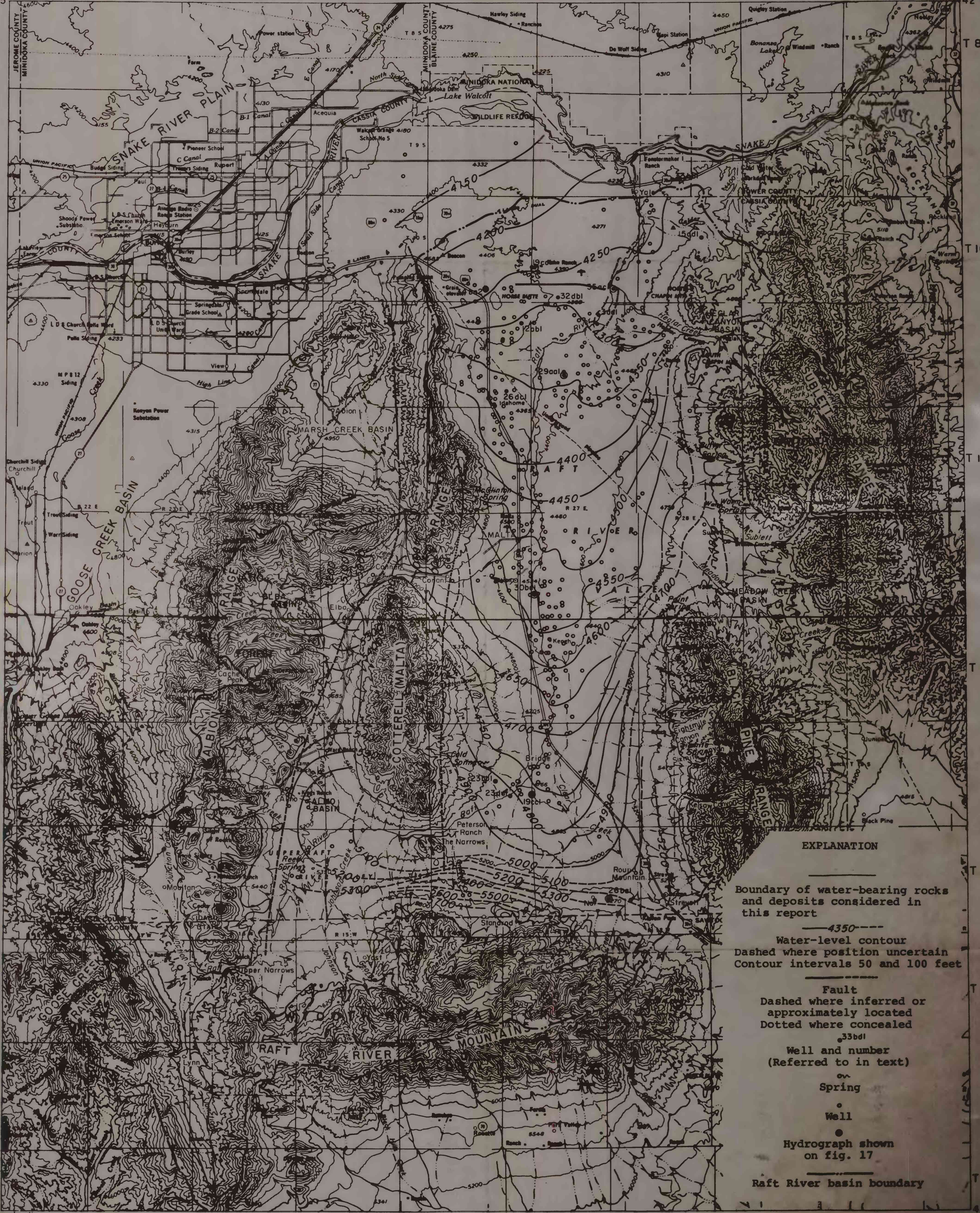
FIGURE 14.--Wells and water-level contours for Raft River basin, Idaho and Utah, spring 1966.
