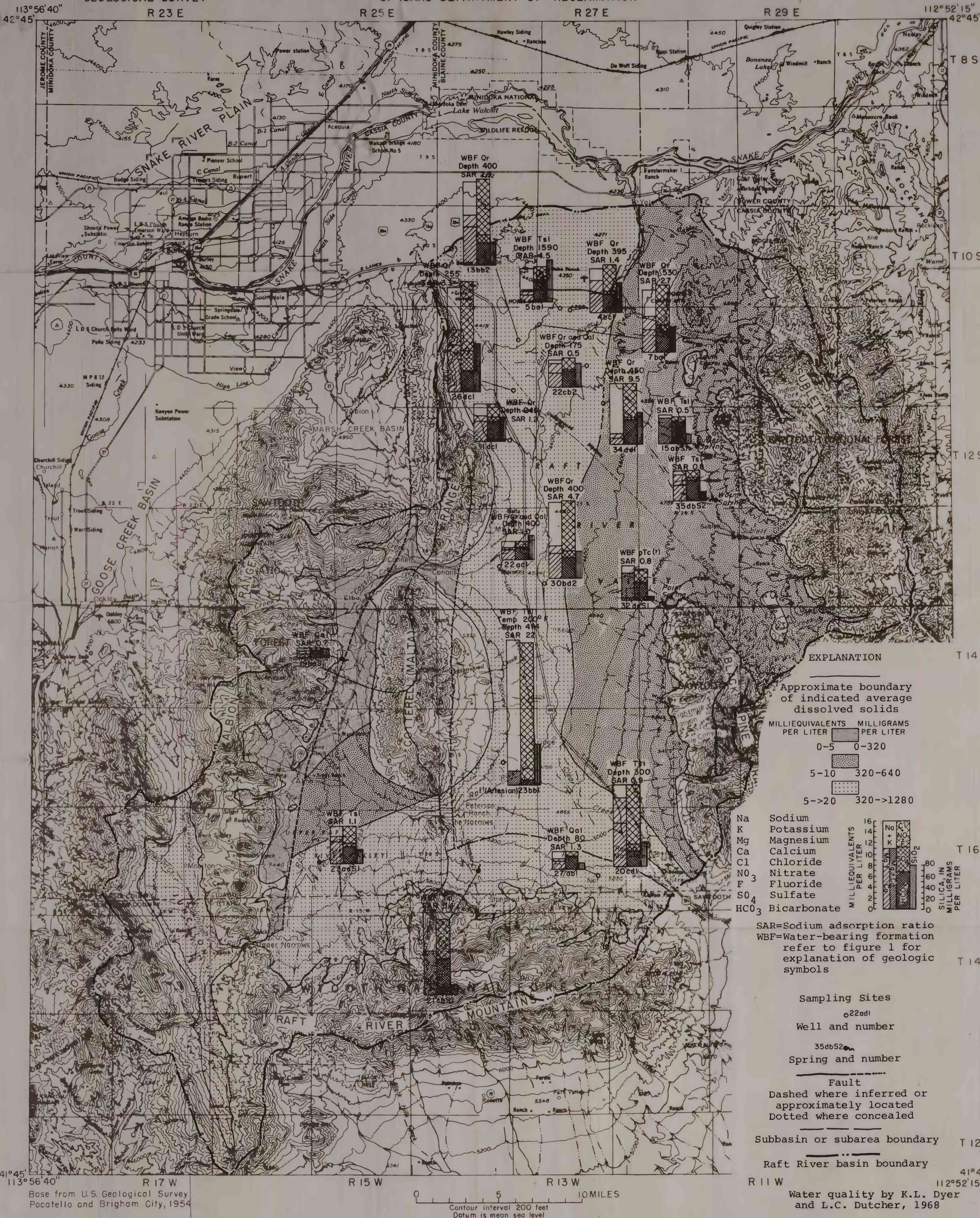
FIGURE 23.--Map showing chemical quality of ground water in the Raft River basin, Idaho and Utah.
