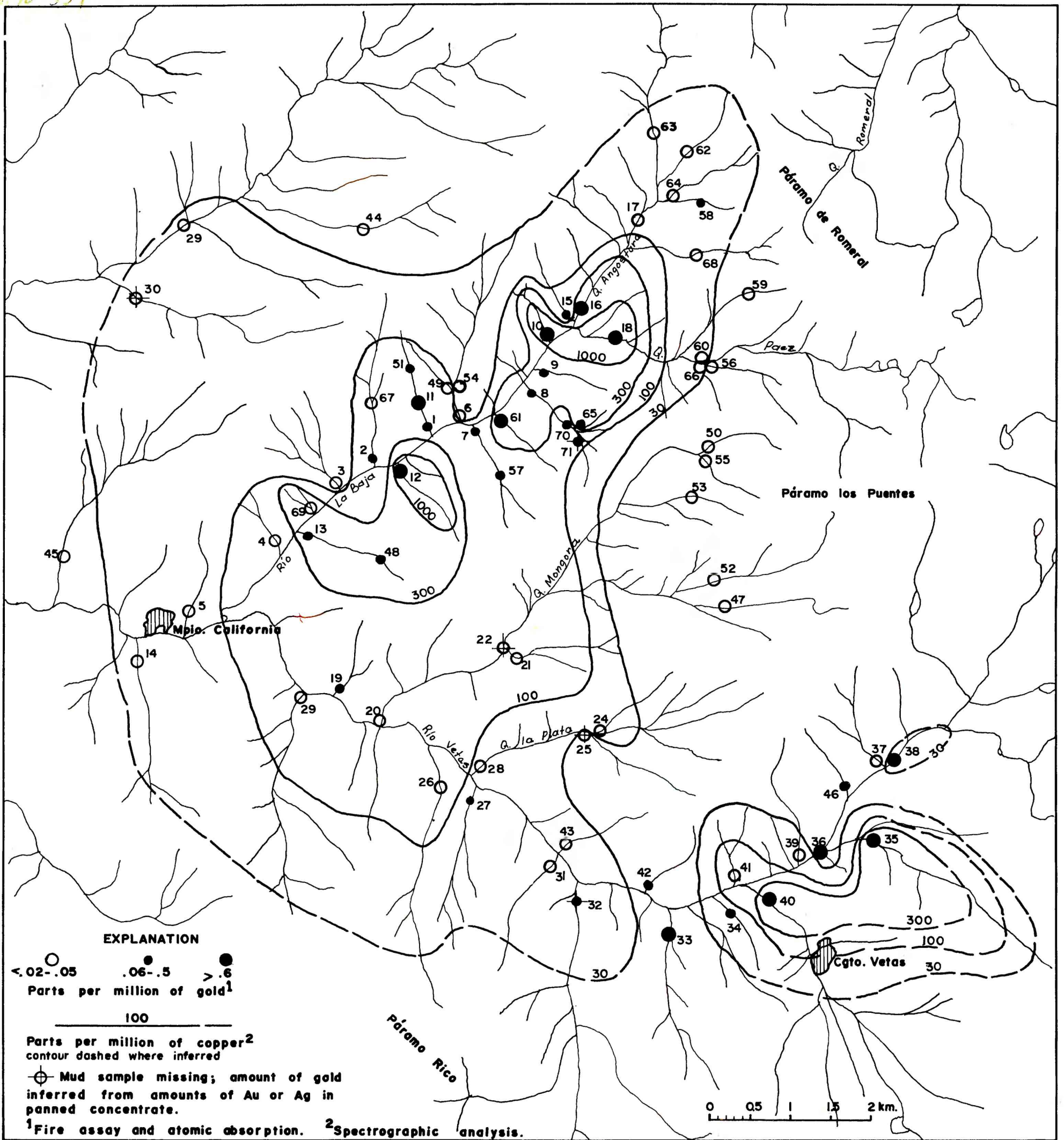
FIGURE 9 : Map showing distribution of gold in mud and copper in panned concentrate of stream sediment, California and Vetas district, Santander, Colombia. Sample data plotted on Figures 7 and 8, further detail given in Table 2.
