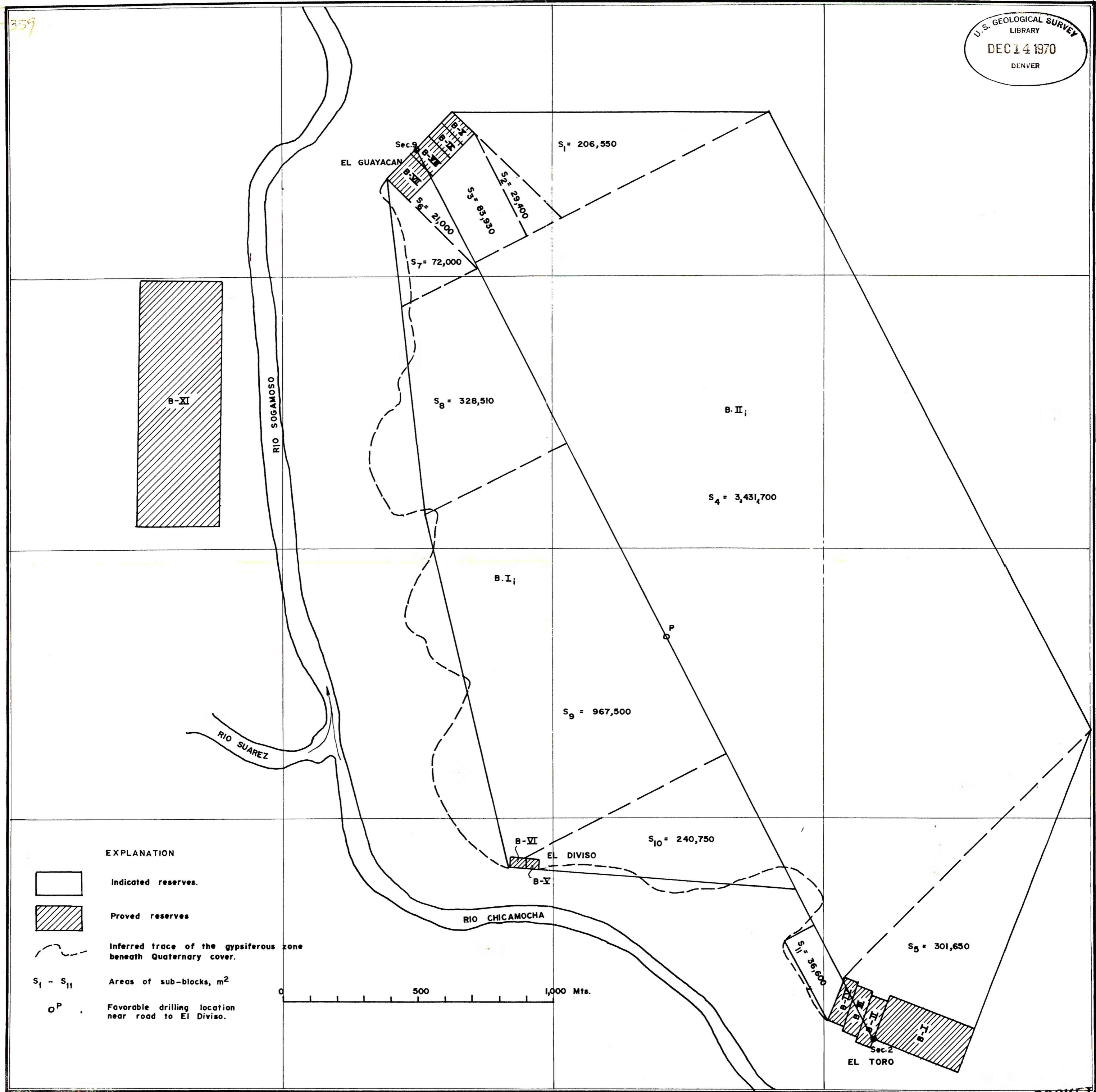
FIGURE 16.-- Sketch map showing blocks of proved and indicated reserves of gypsum on the Mesa de las Santas.
