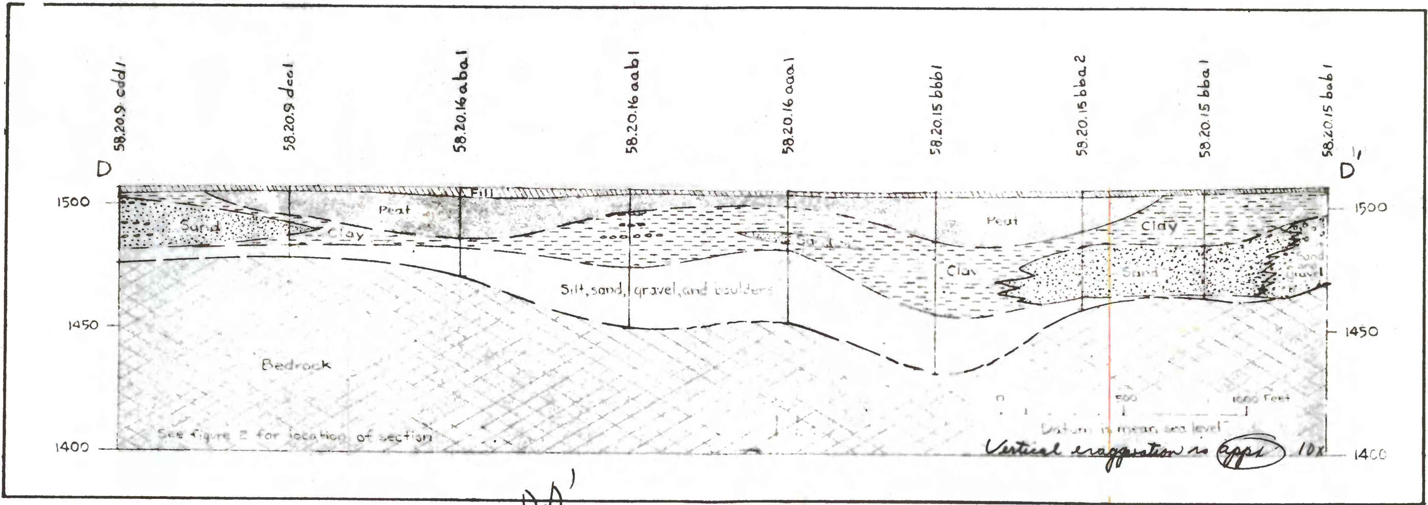
FIGURE 8. — GEOLOGIC SECTION D-D' THROUGH SWAMP NORTH OF CHISHOLM.
