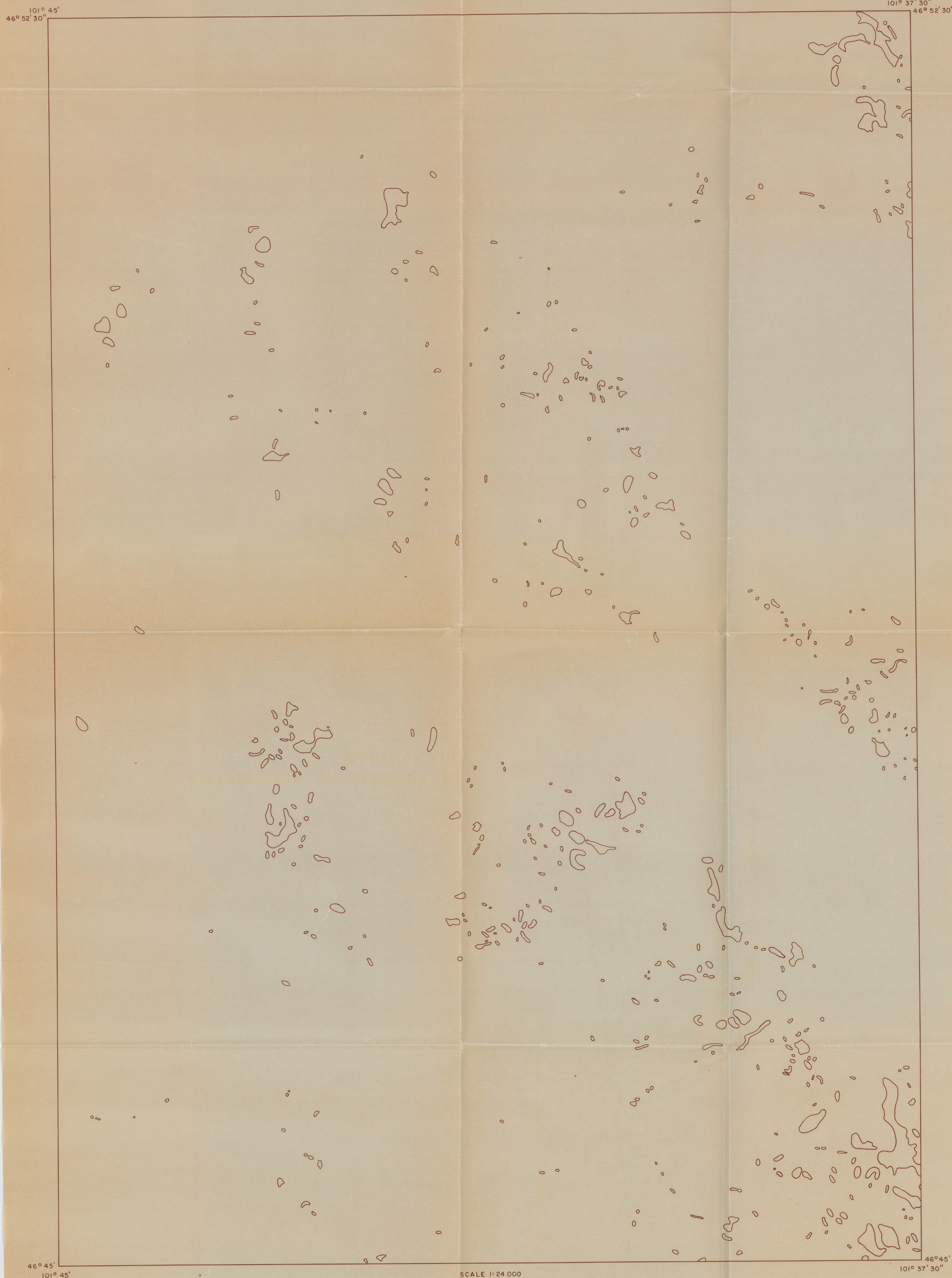
DISTRIBUTION OF GANISTER BLOCKS IN THE DENGATE QUADRANGLE, MORTON COUNTY, NORTH DAKOTA
