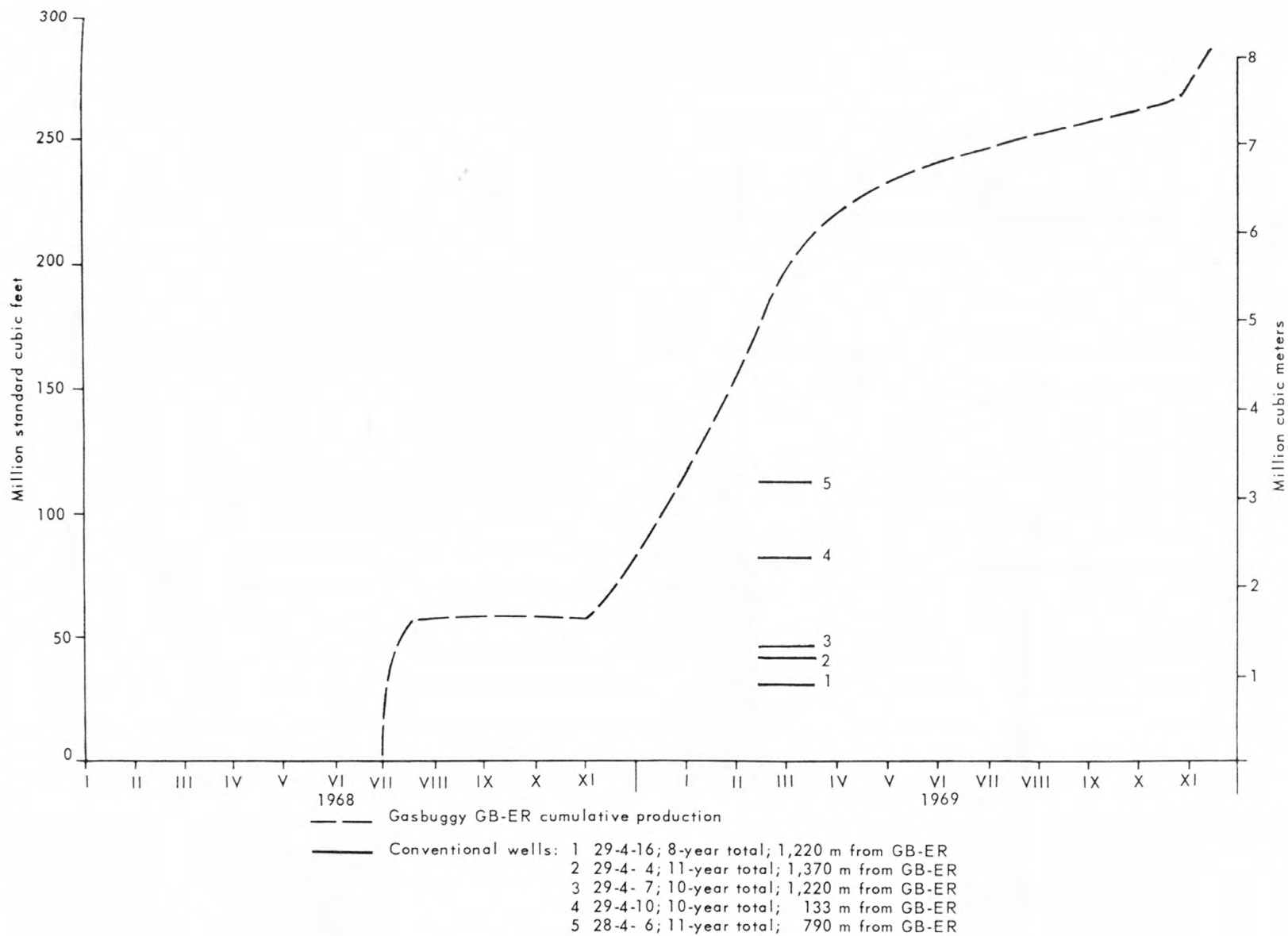
Figure 11. Production history of the Gasbuggy site (After Holzer, 1970)
