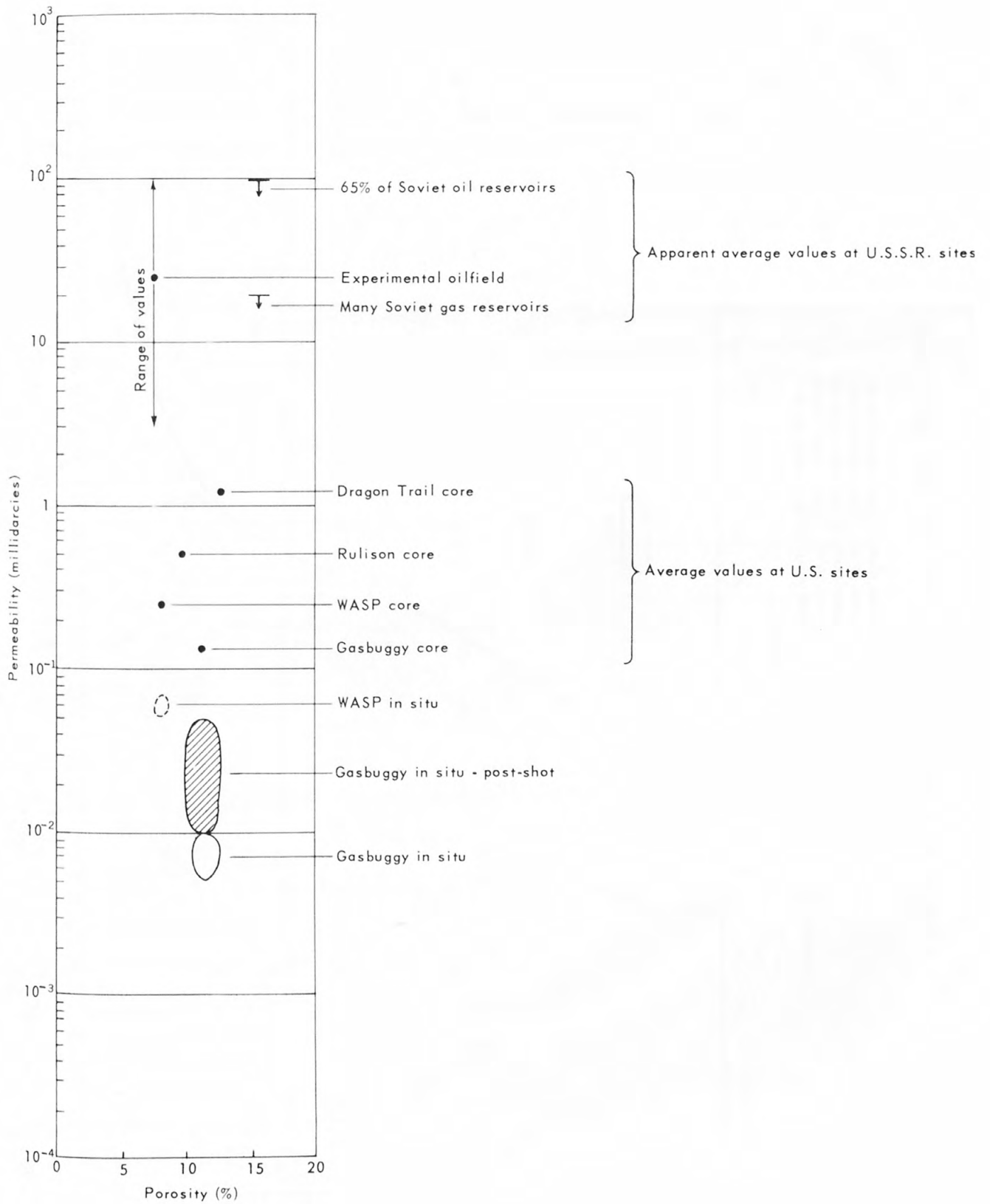
Figure 10. Core permeability and petroleum-stimulation project sites
