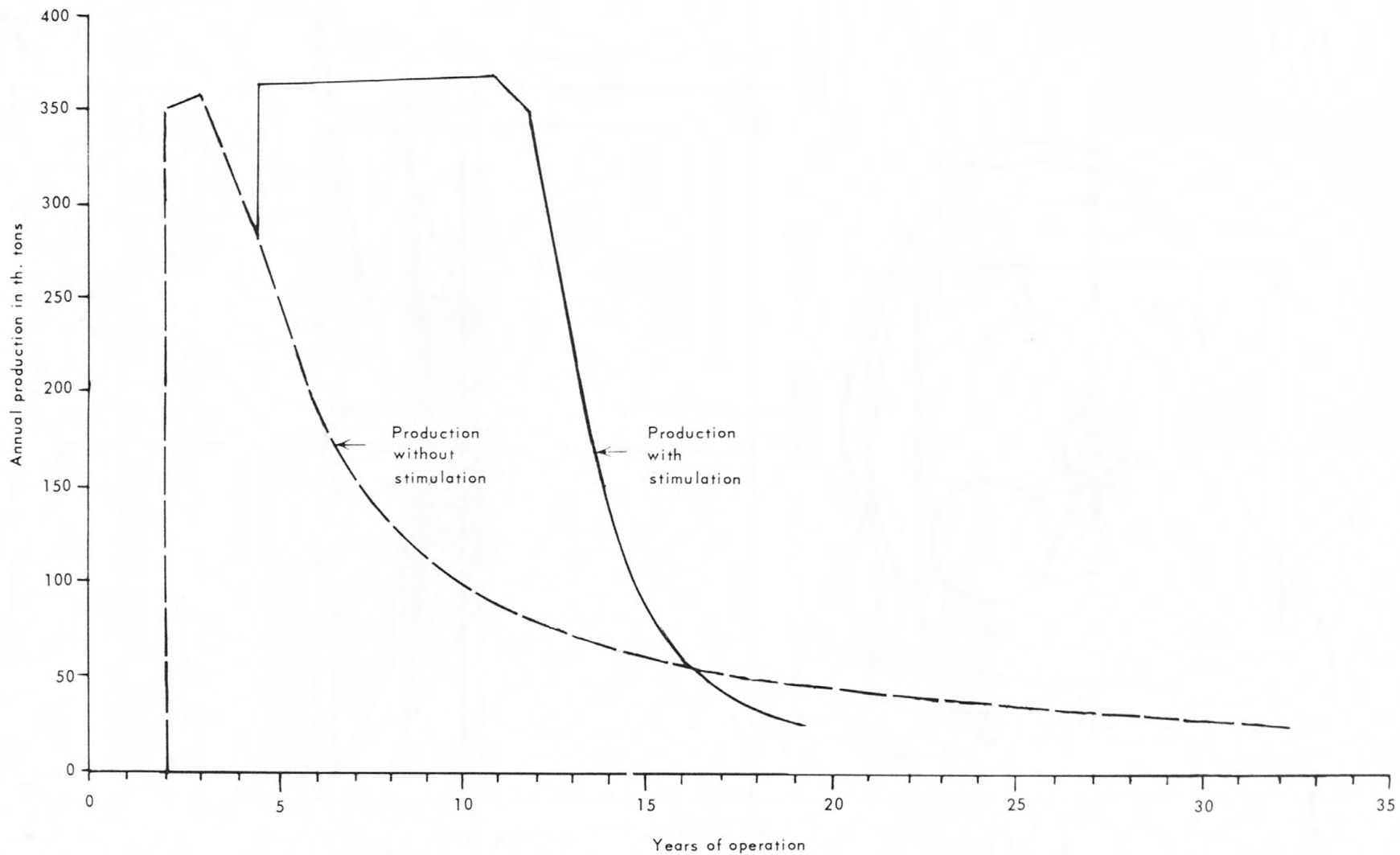
Figure 24. Production history of water-drive oilfield project site - Scheme II (After Kedrovskiy, 1970)
