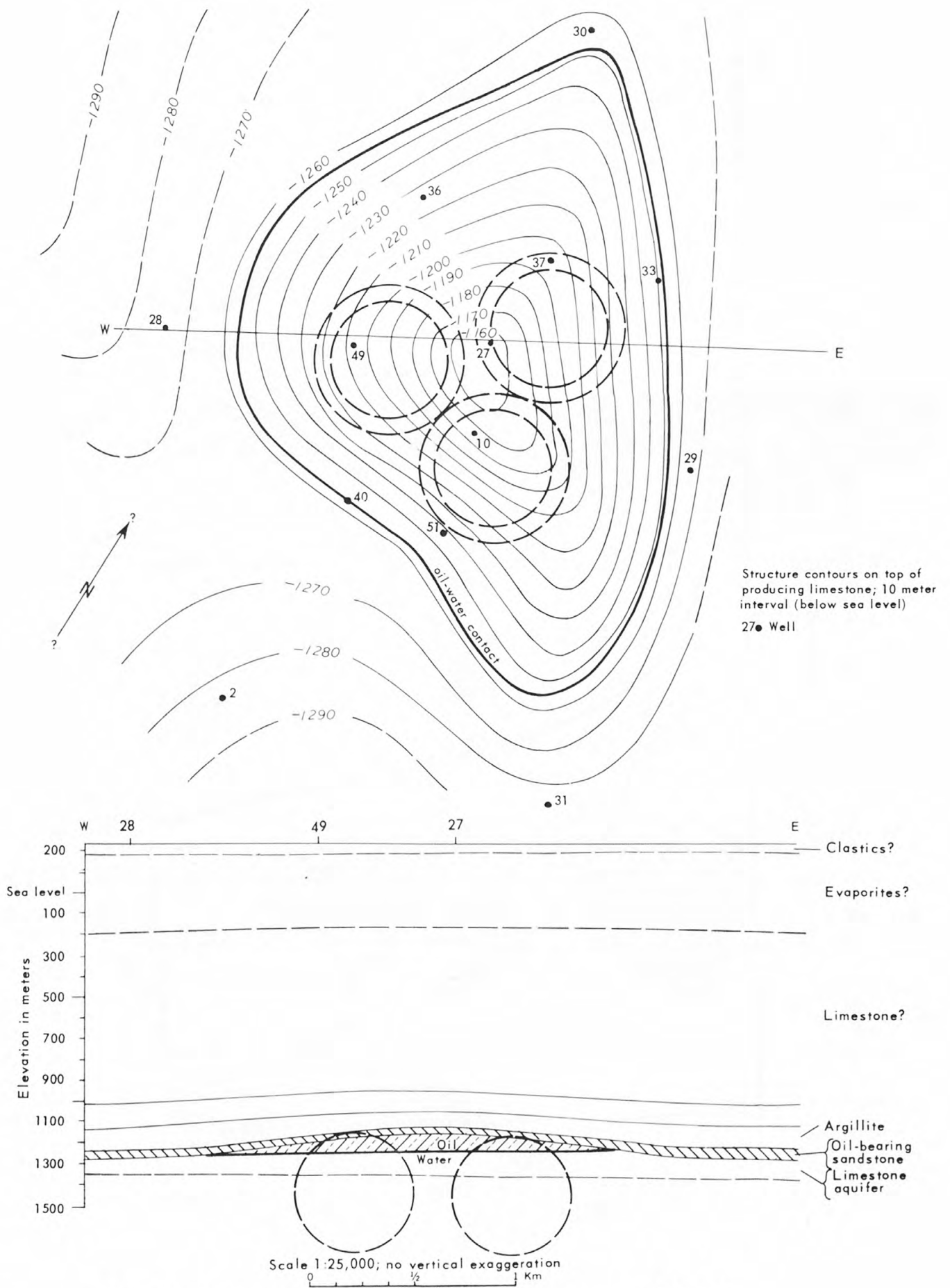
Figure 23. Subsurface geology of water-drive oilfield project site - Scheme II (After Kedrovskiy, 1970)
