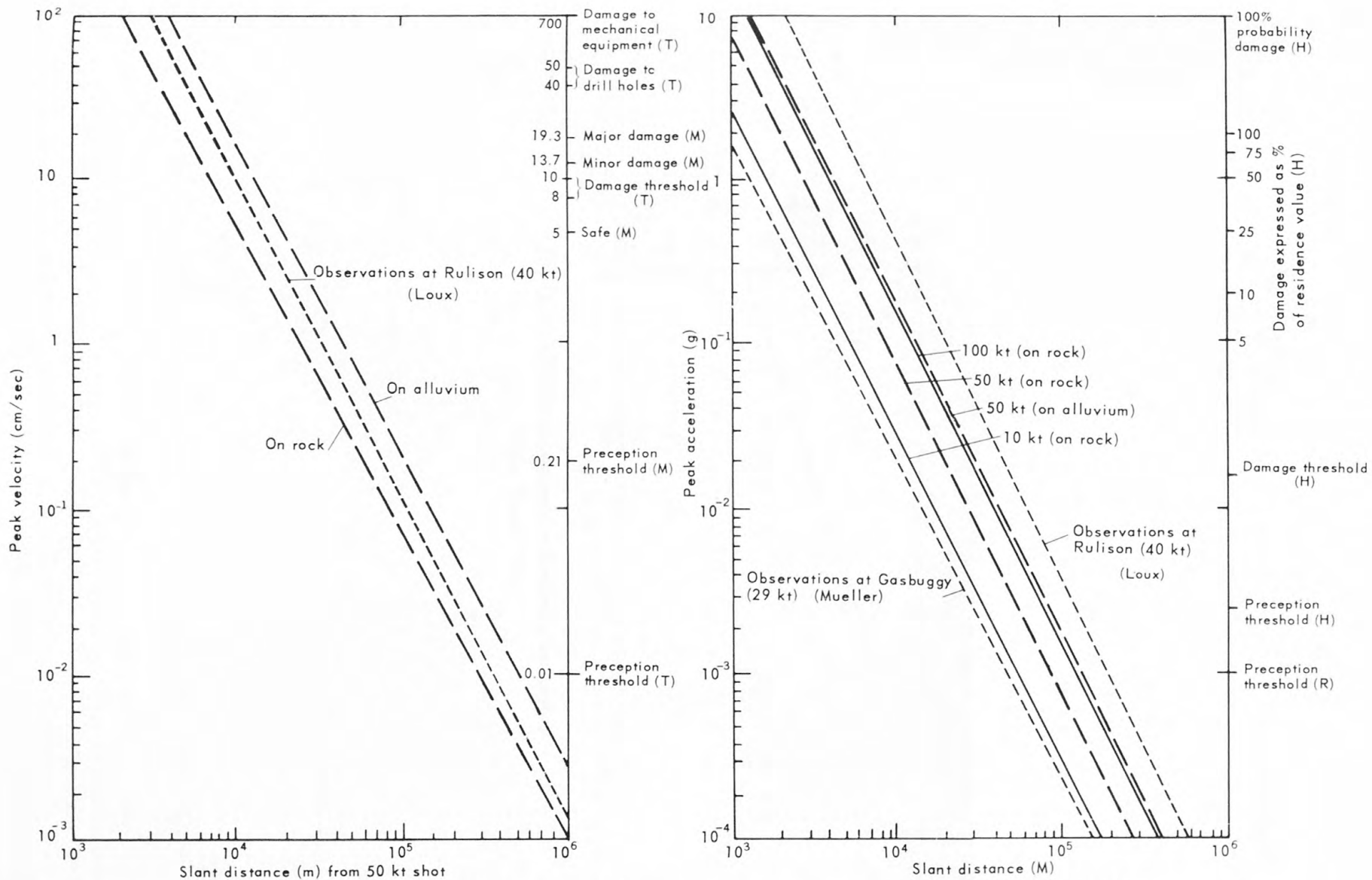
Figure 17. Predicted peak surface particle motion versus slant distance (From Kinnamon et al, 1967) Damage evaluations from (R) Richter, 1958; (M) Mickey, 1964; (H) Hughes, 1968; (T) Teller et al, 1968 Observed motion from Mueller, 1970, and Loux, 1970
