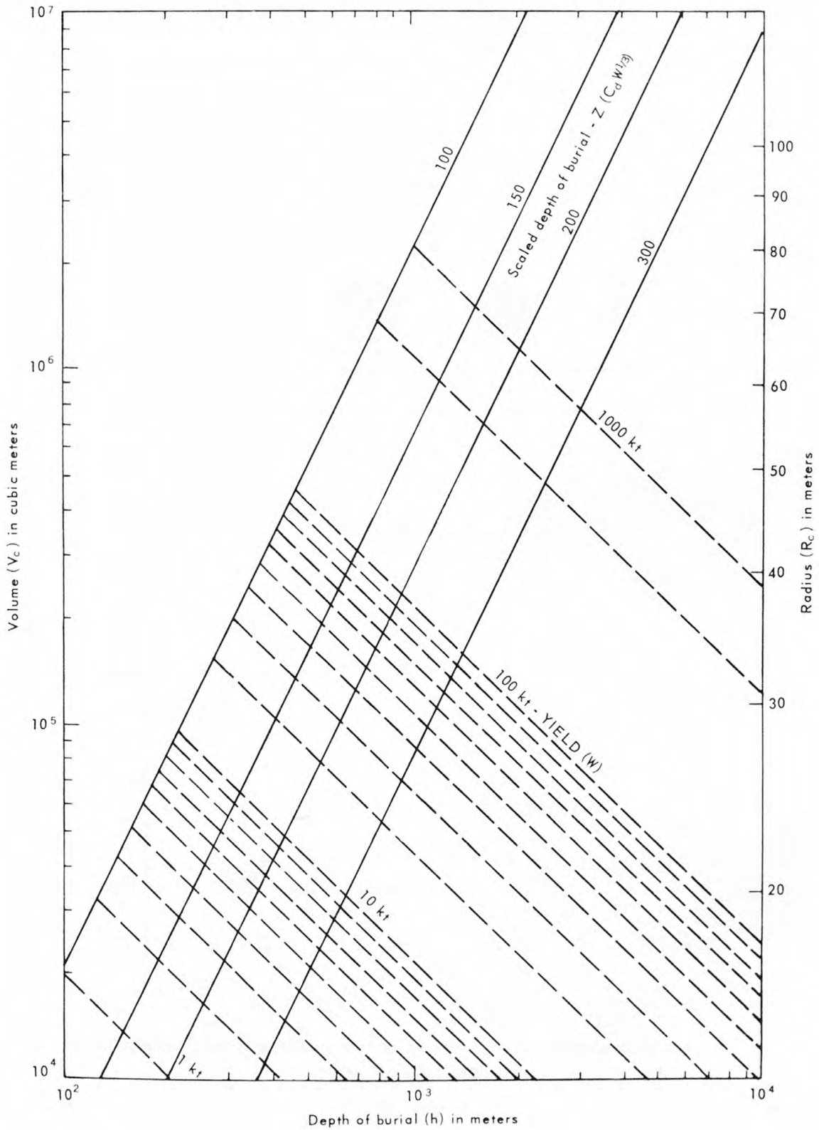
Figure 2. Relationships of yield, depth, and cavity radius and volume in granite (After Lewis, 1970)
