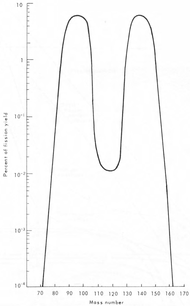
Figure 15. Yield-mass curve for thermal fission of U^{235} (From Miskel, 1964)
