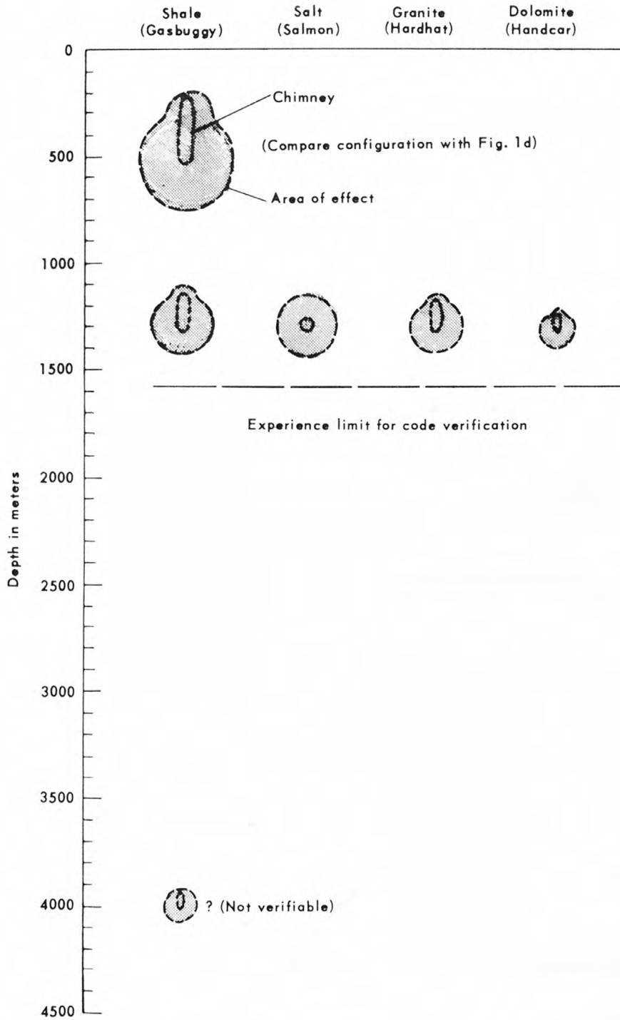
Figure 3. Effects of rock mechanics on underground nuclear explosions (After Nordyke, 1970)
