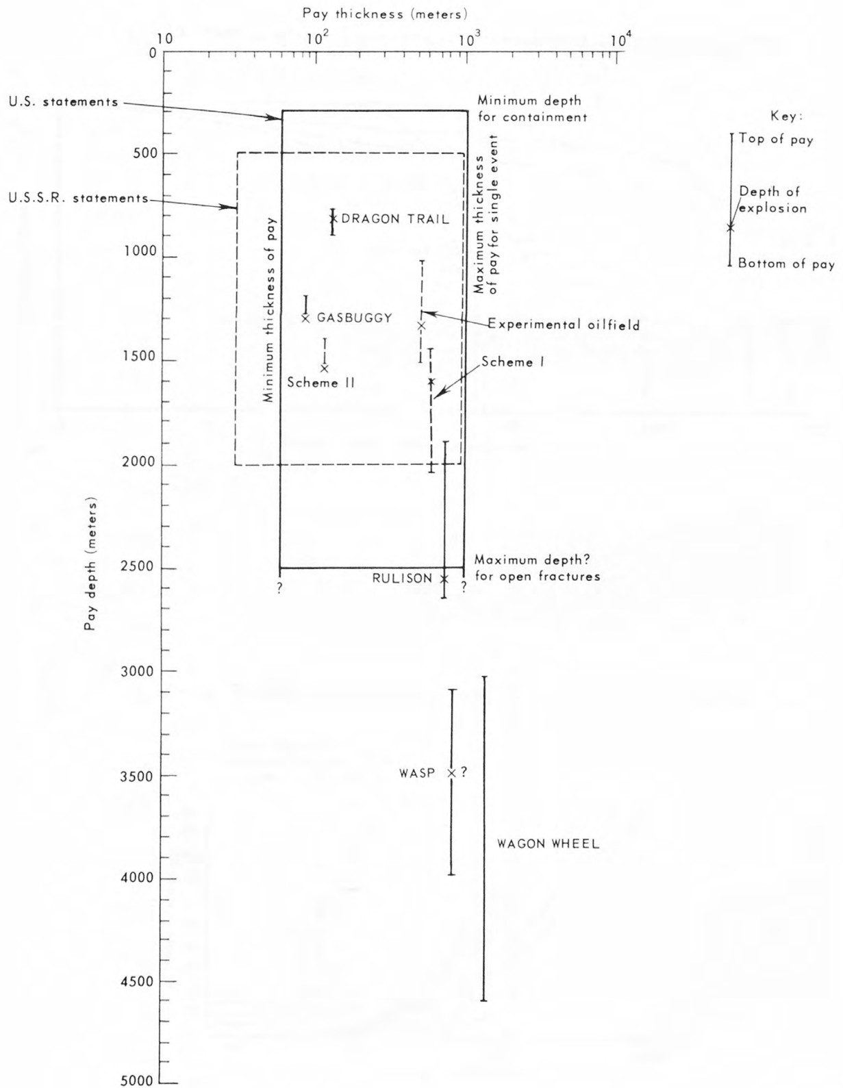
Figure 12. Reservoir geometry and petroleum-stimulation amenability
