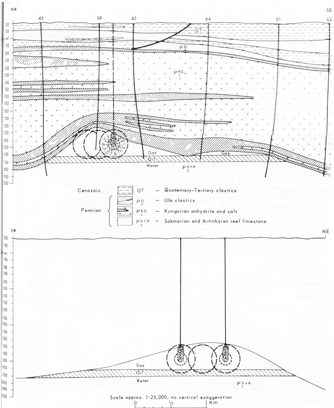
Figure 22. Cross-sections of gasfield project site - Scheme I (After Kedrovskiy, 1970)
