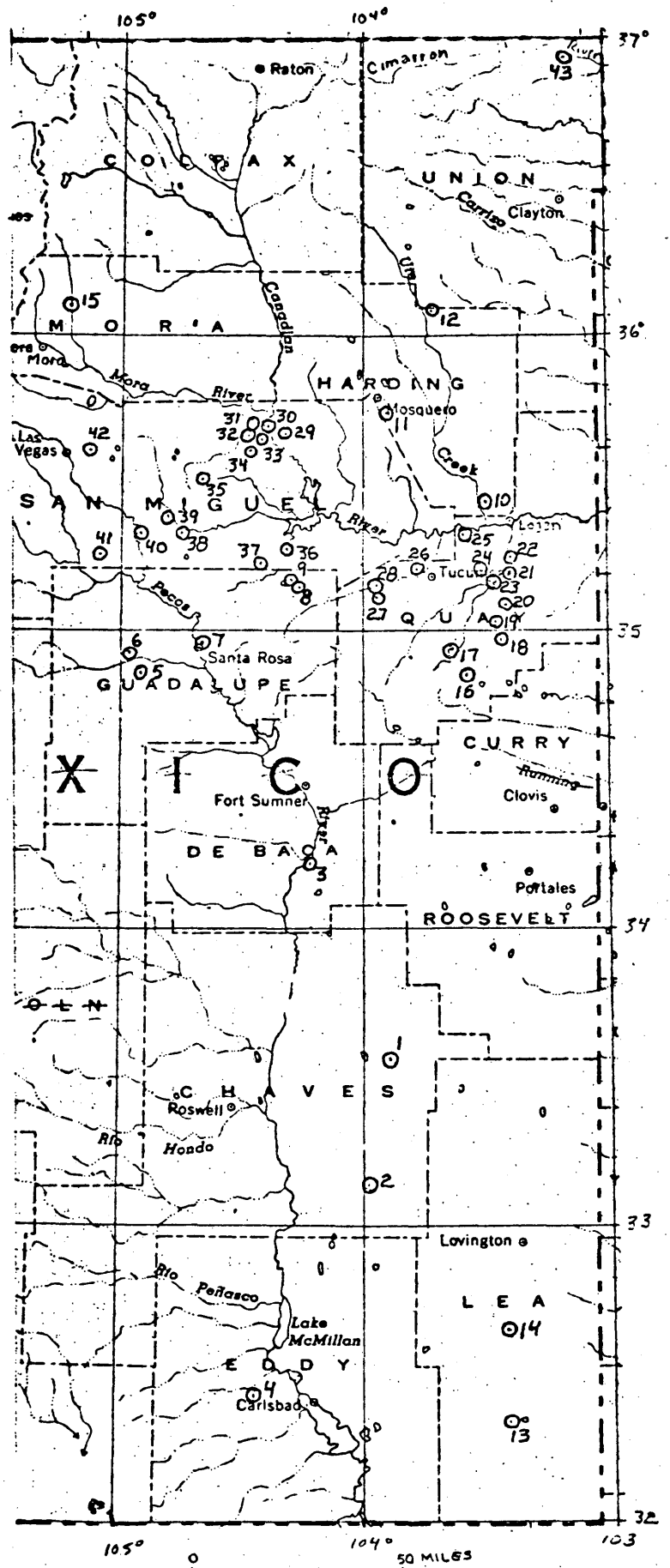
Figure 1.-- Index map of uranium localities in eastern New Mexico
