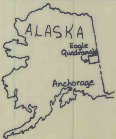
Figure 2. Map of Eagle quadrangle, Alaska, showing localities where analyzed rock samples were collected in 1971.
